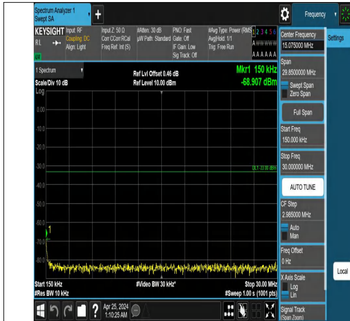
Band2_20MHz_QPSK_19100_1RB#99_0.15~30_0.15~30
