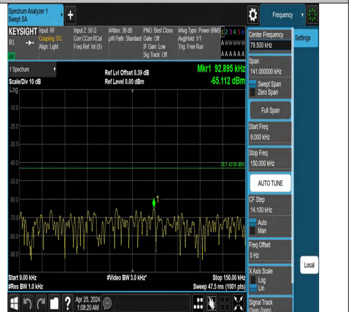
Band2_20MHz_QPSK_18700_1RB#99_0.009~0.15_0.009~0.15
