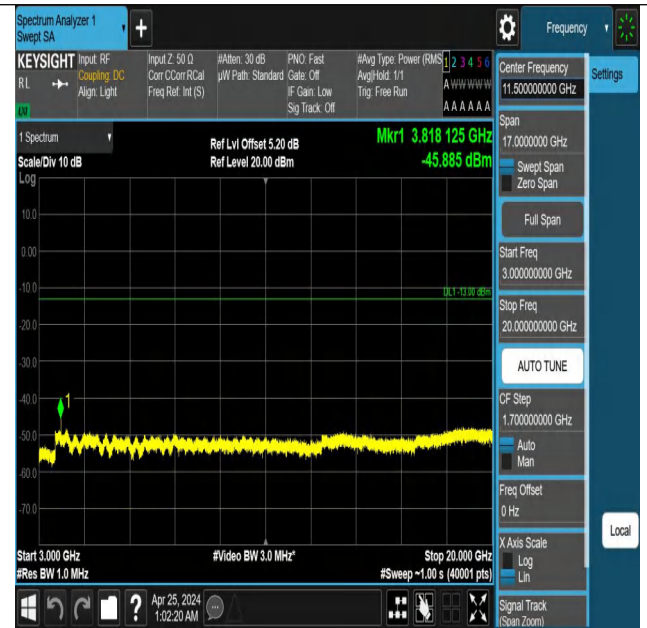
Band2_15MHz_QPSK_19125_1RB#74_3000~20000_3000~20000
