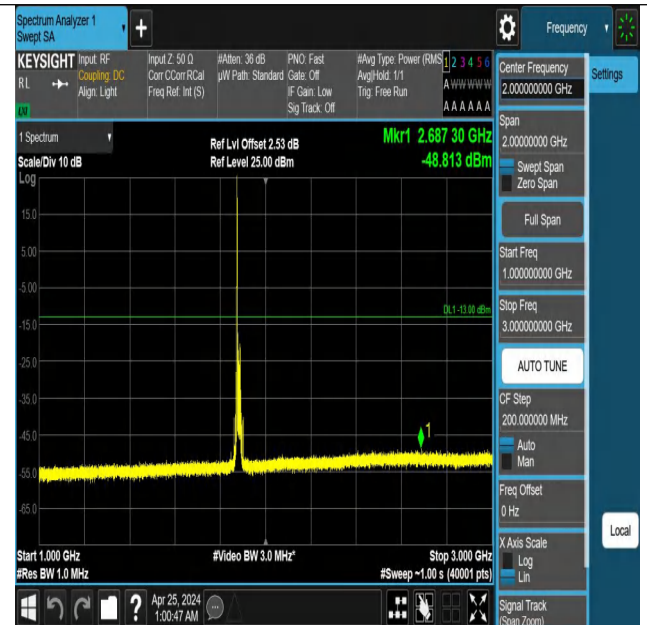
Band2_15MHz_QPSK_18900_1RB#0_1000~3000_1000~3000
