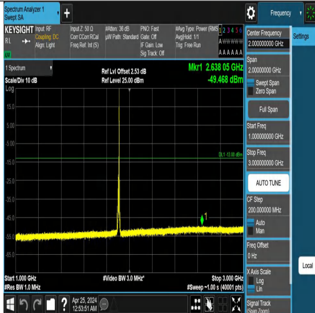
Band2_10MHz_QPSK_19150_1RB#49_1000~3000_1000~3000
