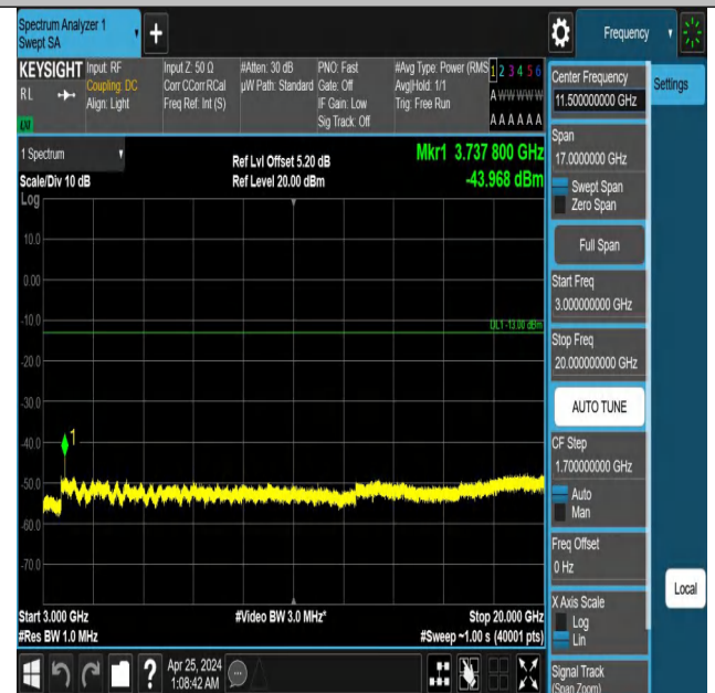
Band2_20MHz_QPSK_18700_1RB#99_3000~20000_3000~20000
