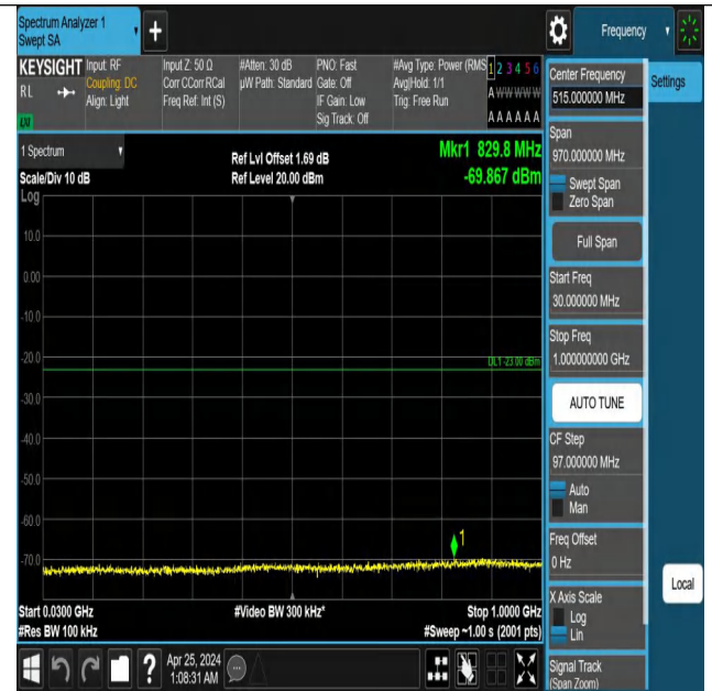
Band2_20MHz_QPSK_18700_1RB#99_30~1000_30~1000
