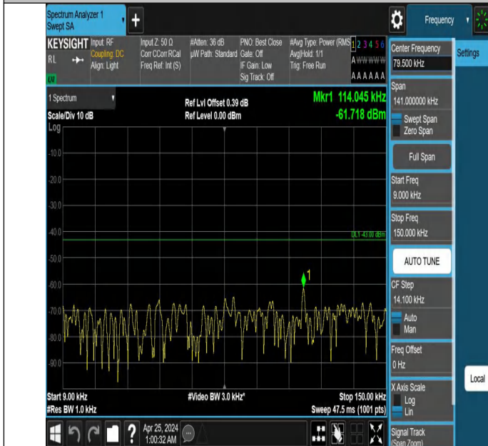
Band2_15MHz_QPSK_18900_1RB#0_0.009~0.15_0.009~0.15
