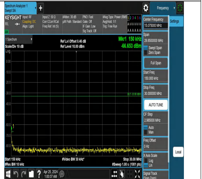
Band2_15MHz_QPSK_18900_1RB#0_0.15~30_0.15~30
