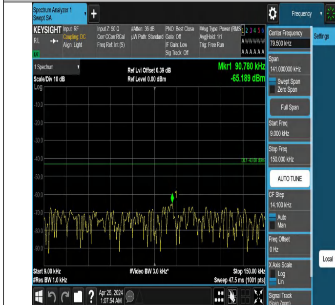
Band2_20MHz_QPSK_18700_1RB#0_0.009~0.15_0.009~0.15
