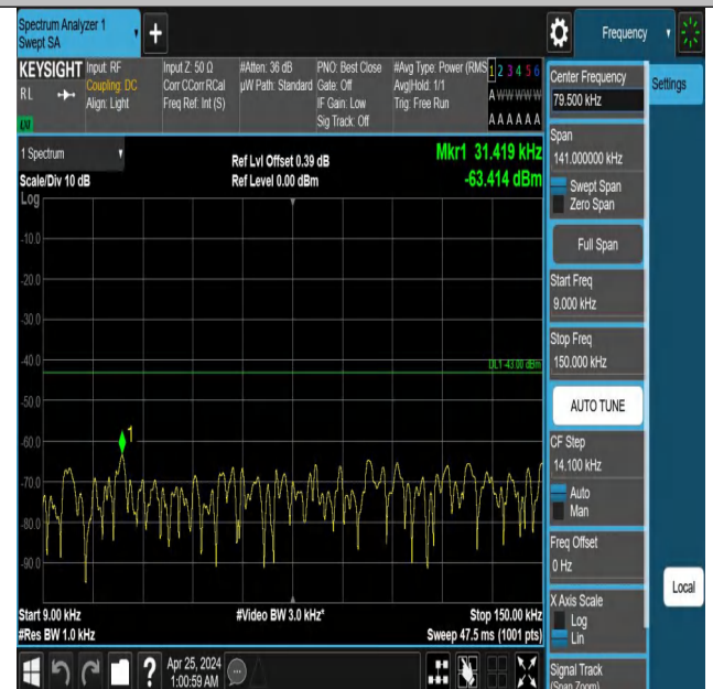
Band2_15MHz_QPSK_18900_1RB#74_0.009~0.15_0.009~0.15
