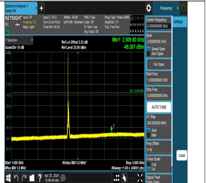
Band2_15MHz_QPSK_18675_1RB#0_1000~3000_1000~3000
