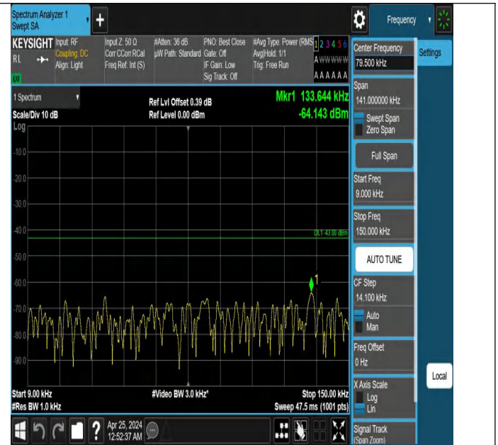
Band2_10MHz_QPSK_18900_1RB#49_0.009~0.15_0.009~0.15
