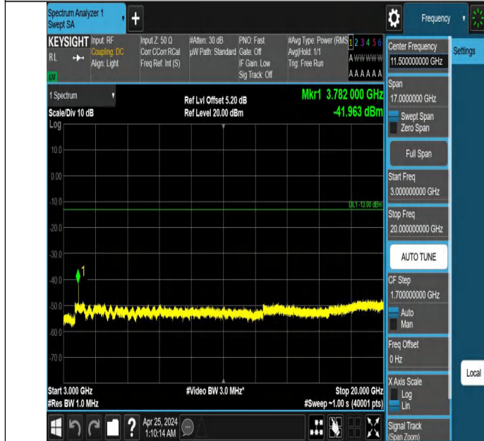
Band2_20MHz_QPSK_19100_1RB#0_3000~20000_3000~20000
