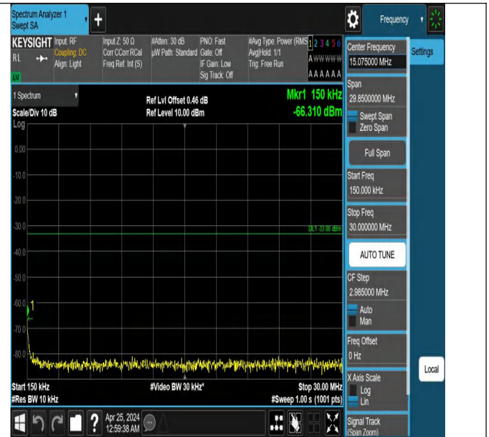
Band2_15MHz_QPSK_18675_1RB#0_0.15~30_0.15~30
