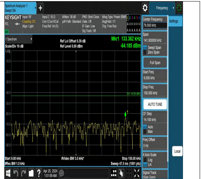
Band2_15MHz_QPSK_19125_1RB#74_0.009~0.15_0.009~0.15
