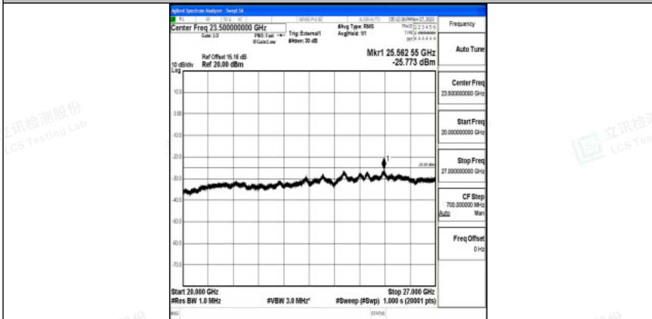
Band41_5MHz_64QAM_41565_1RB#0_20000~27000_20000~27000
