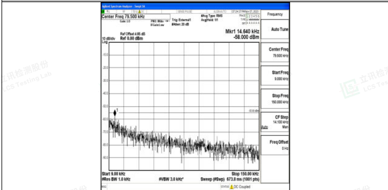
Band41_15MHz_64QAM_39725_1RB#0_0.009~0.15_0.009~0.15
