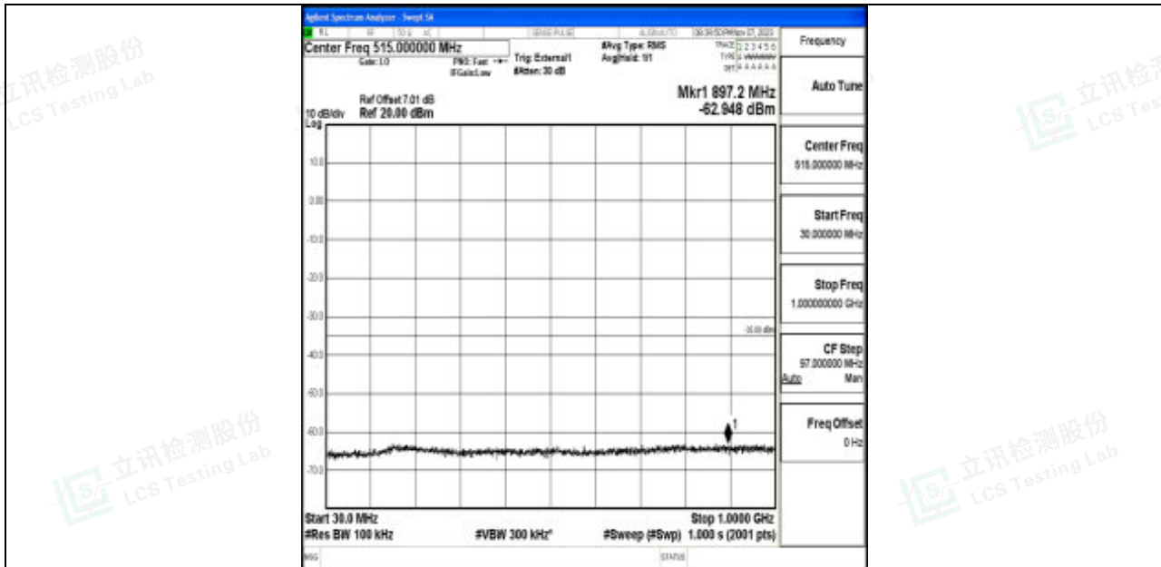
Band41_20MHz_64QAM_41490_1RB#0_30~1000_30~1000
