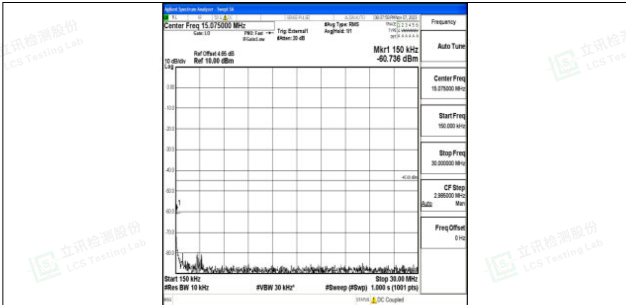
Band41_20MHz_16QAM_41490_1RB#0_0.15~30_0.15~30
