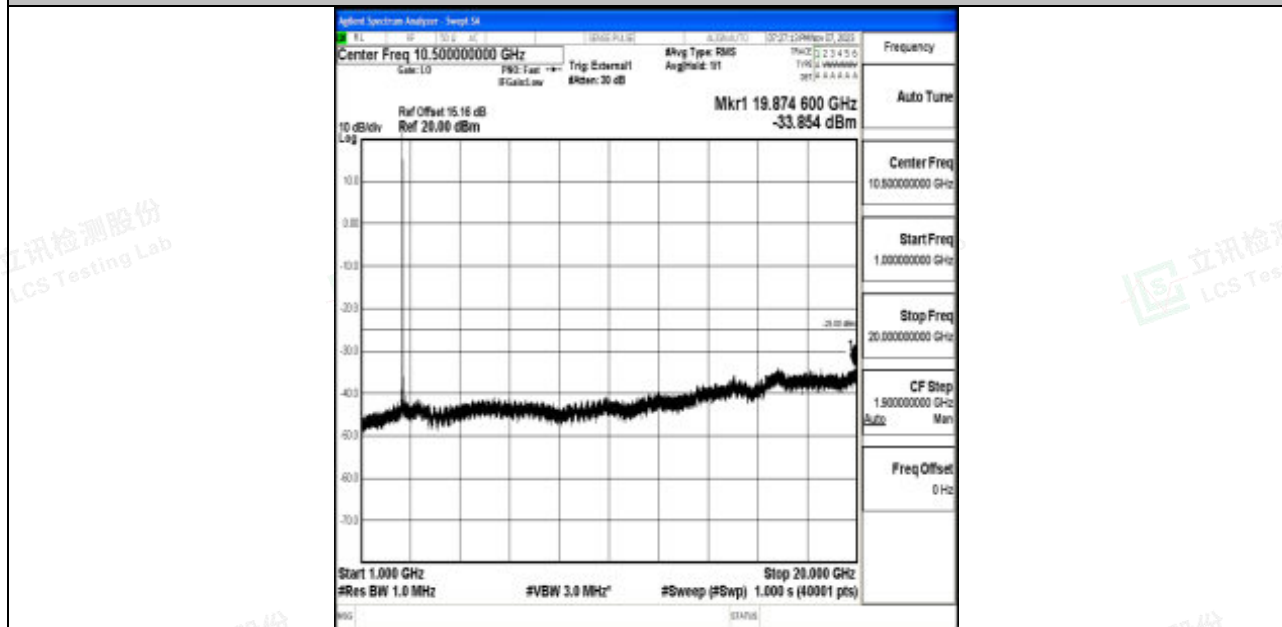
Band41_15MHz_QPSK_40620_1RB#0_1000~20000_1000~20000
