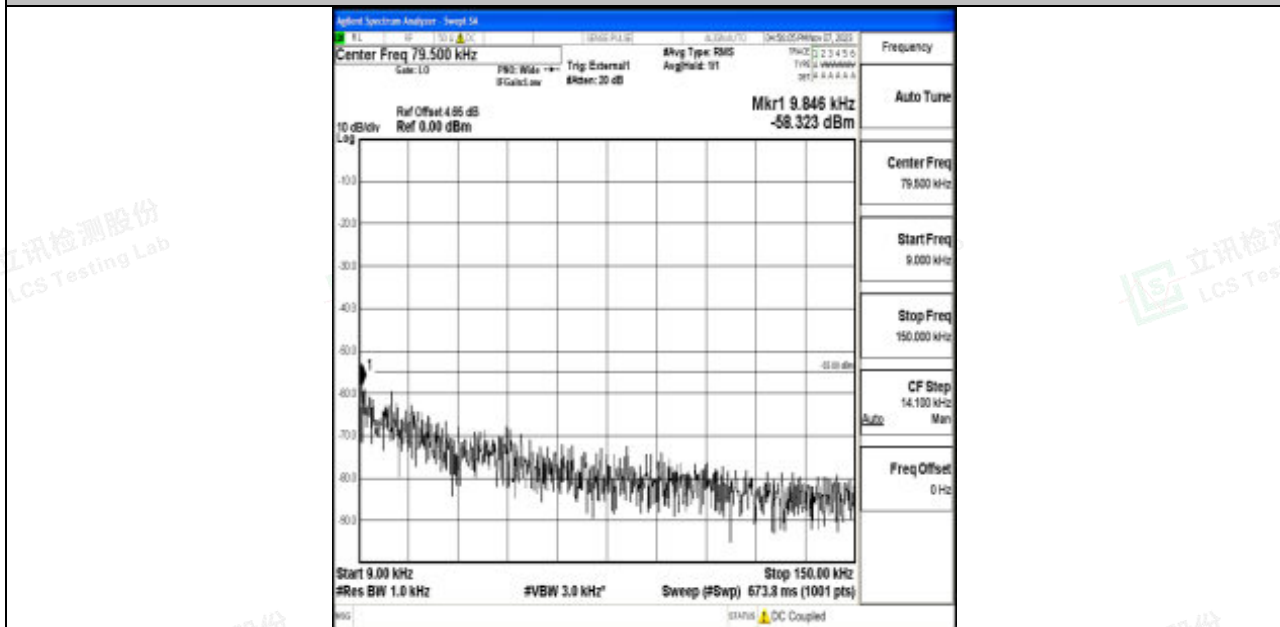
Band41_5MHz_64QAM_39675_1RB#0_0.009~0.15_0.009~0.15
