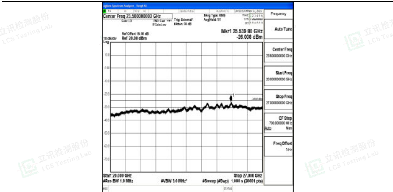
Band41_5MHz_16QAM_39675_1RB#0_20000~27000_20000~27000
