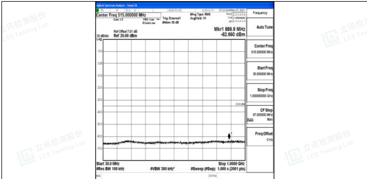
Band41_15MHz_16QAM_39725_1RB#0_30~1000_30~1000
