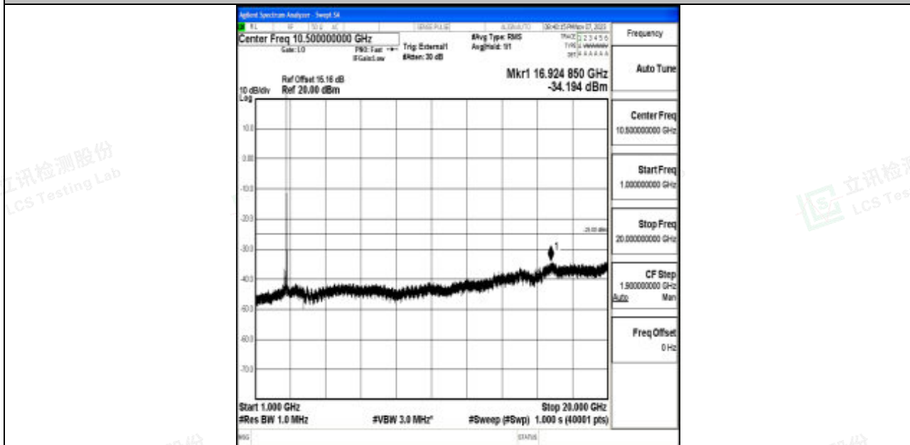
Band41_20MHz_64QAM_41490_1RB#0_1000~20000_1000~20000
