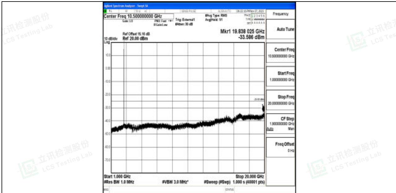
Band41_10MHz_64QAM_40620_1RB#0_1000~20000_1000~20000
