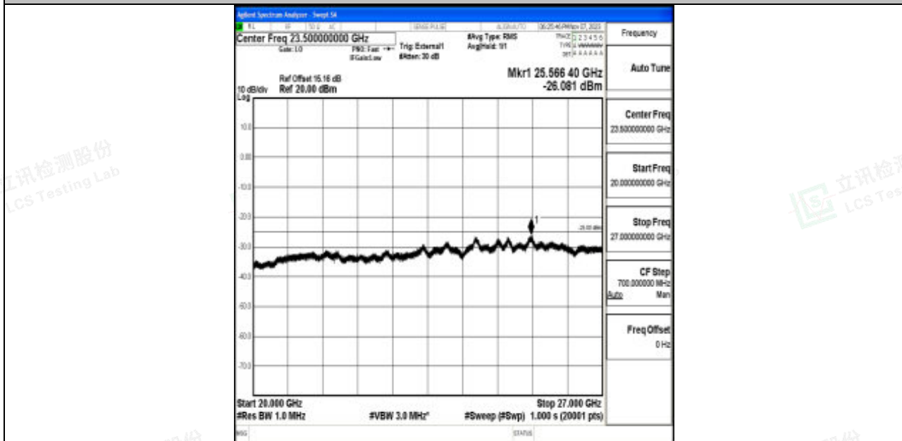
Band41_10MHz_16QAM_41540_1RB#0_20000~27000_20000~27000
