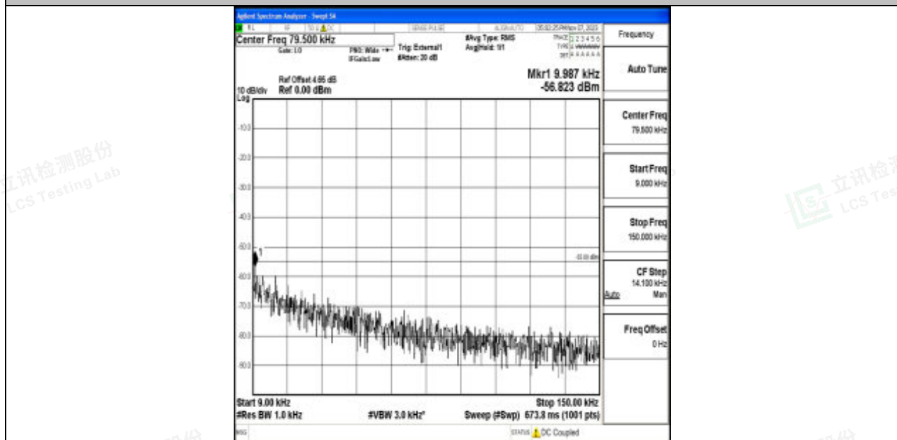
Band41_5MHz_QPSK_41565_1RB#0_0.009~0.15_0.009~0.15
