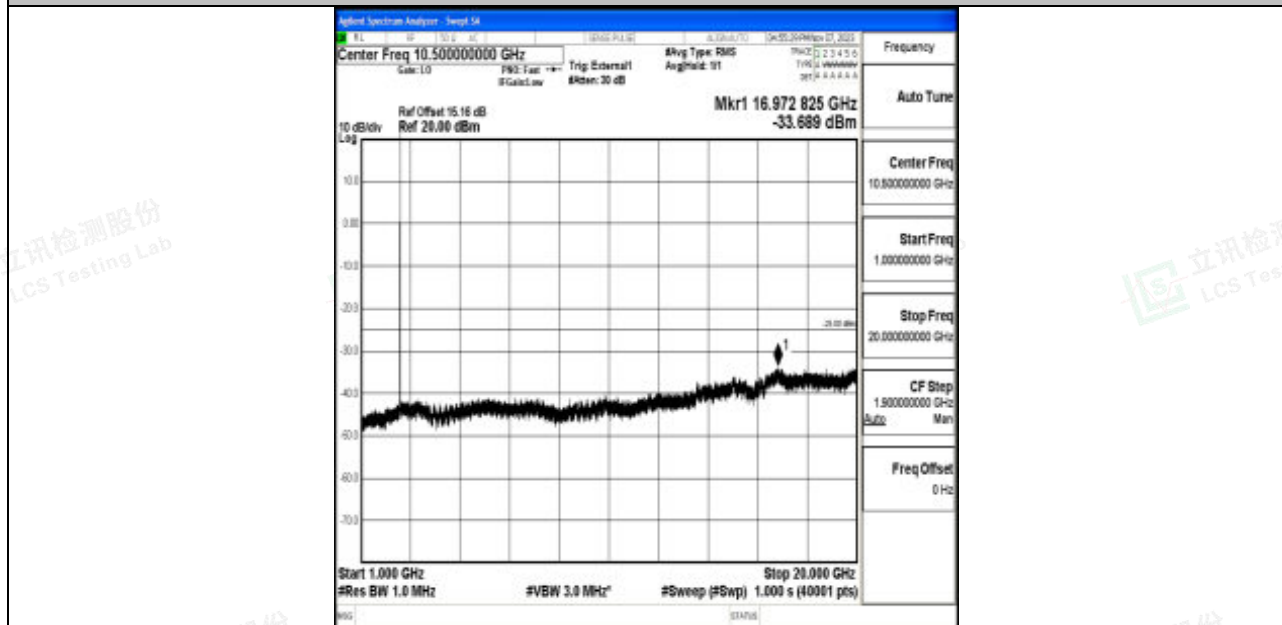
Band41_5MHz_16QAM_39675_1RB#0_1000~20000_1000~20000
