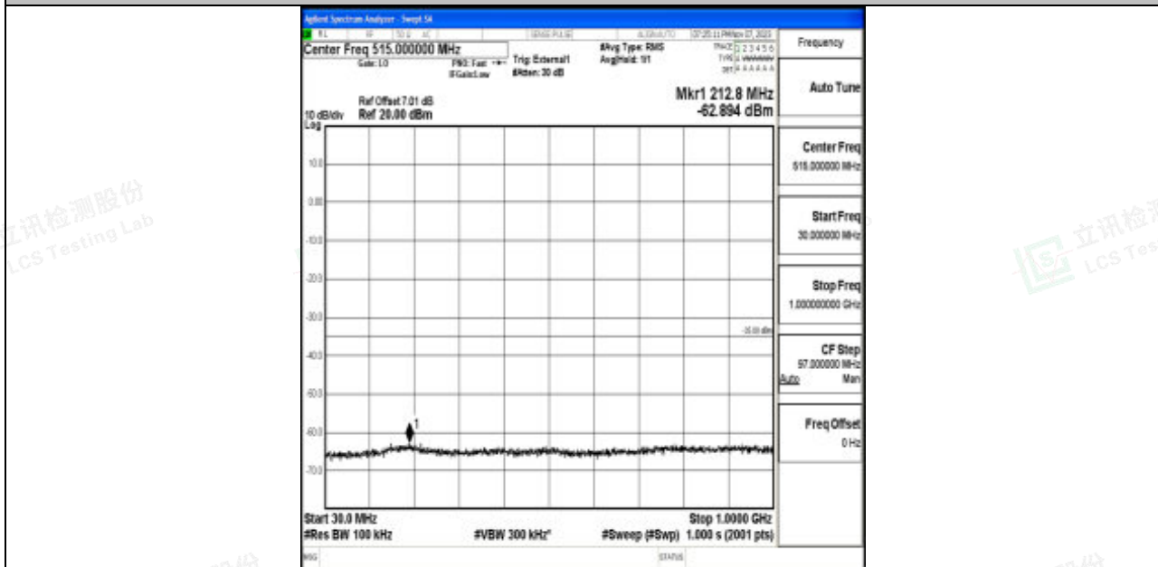
Band41_15MHz_64QAM_39725_1RB#0_30~1000_30~1000
