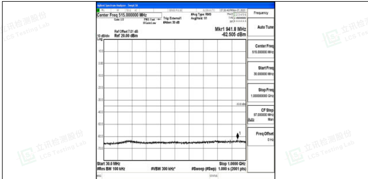
Band41_15MHz_QPSK_40620_1RB#0_30~1000_30~1000
