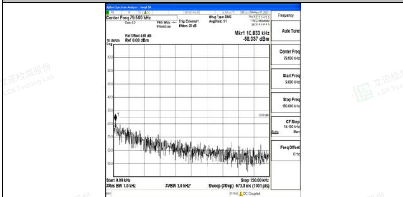
Band41_5MHz_64QAM_41565_1RB#0_0.009~0.15_0.009~0.15
