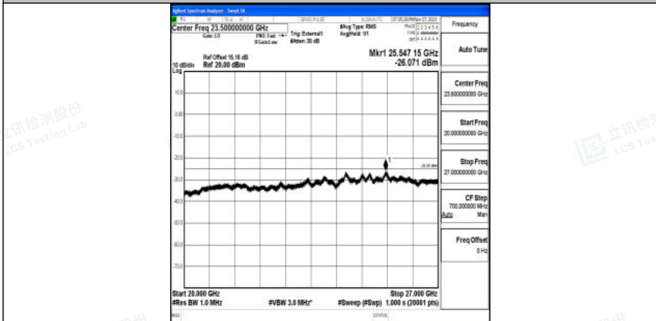
Band41_15MHz_64QAM_41515_1RB#0_20000~27000_20000~27000
