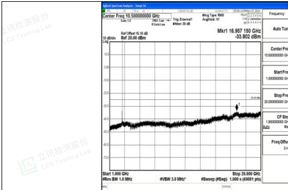
Band41_5MHz_16QAM_40620_1RB#0_1000~20000_1000~20000
