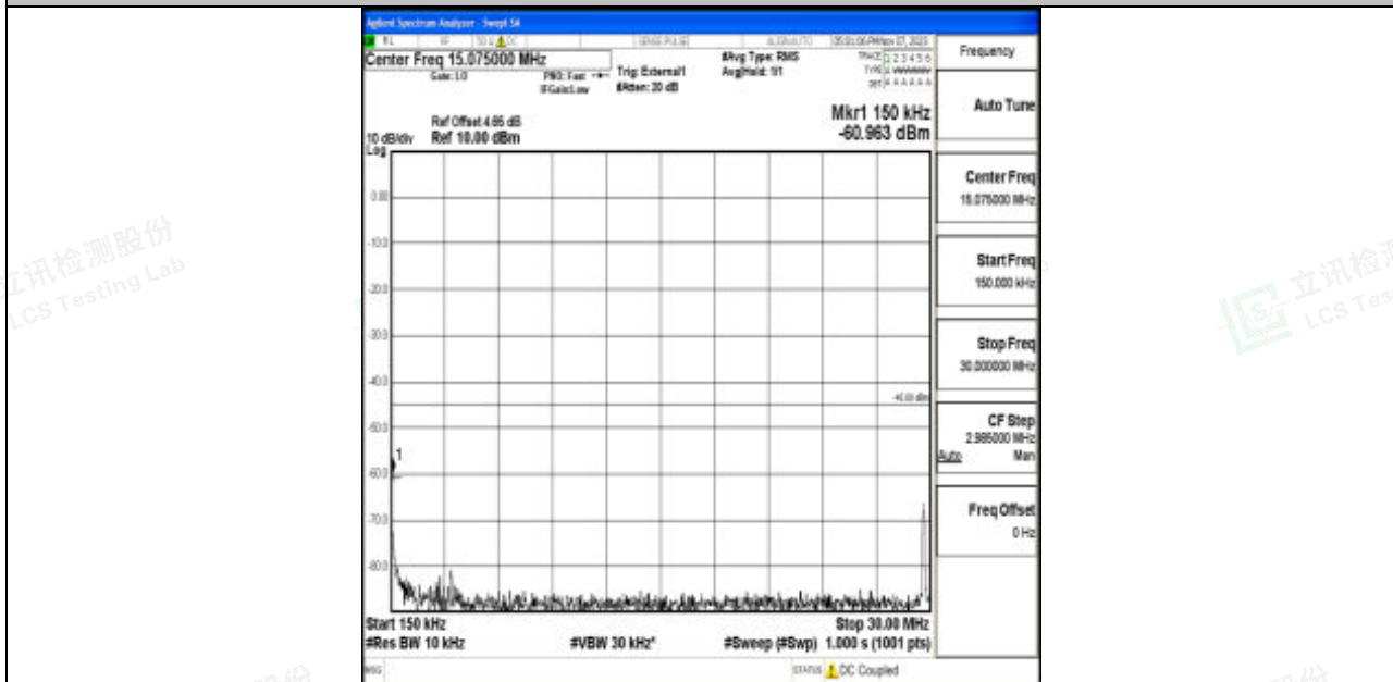
Band41_5MHz_64QAM_40620_1RB#0_0.15~30_0.15~30
