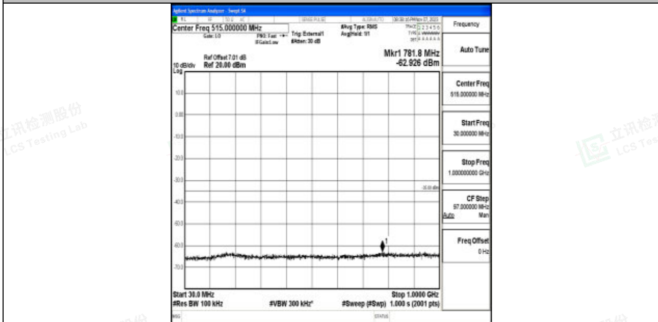
Band41_20MHz_16QAM_41490_1RB#0_30~1000_30~1000
