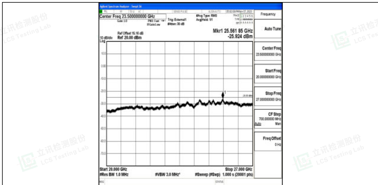
Band41_5MHz_64QAM_40620_1RB#0_20000~27000_20000~27000
