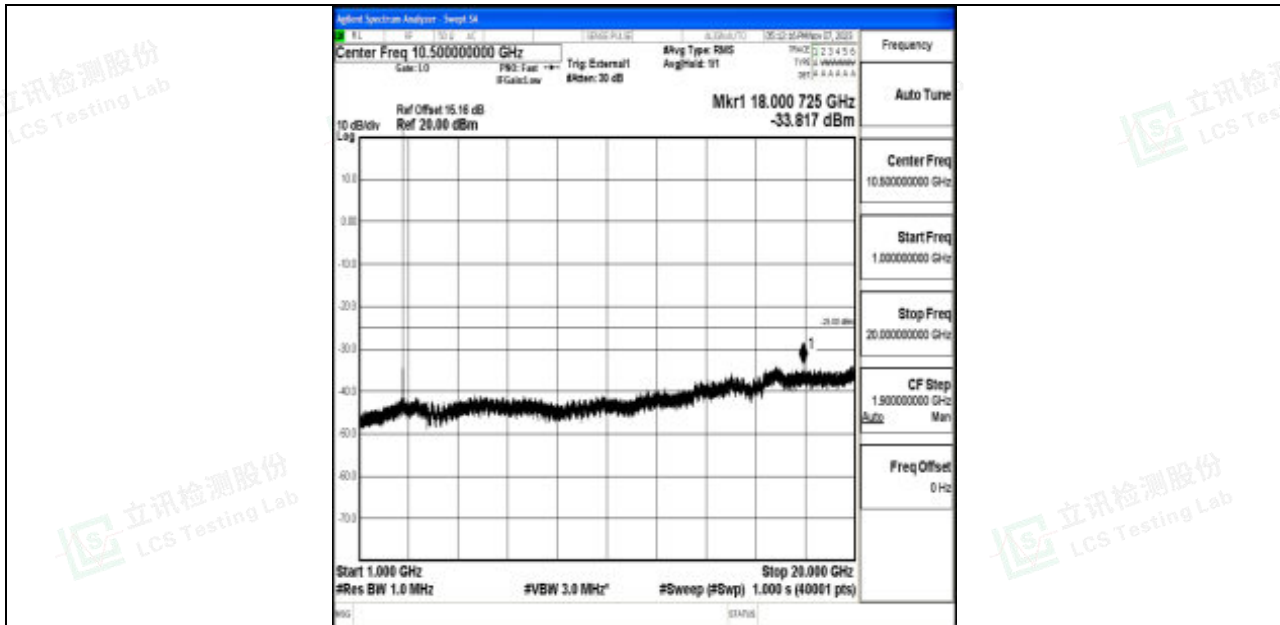
Band41_5MHz_64QAM_41565_1RB#0_1000~20000_1000~20000
