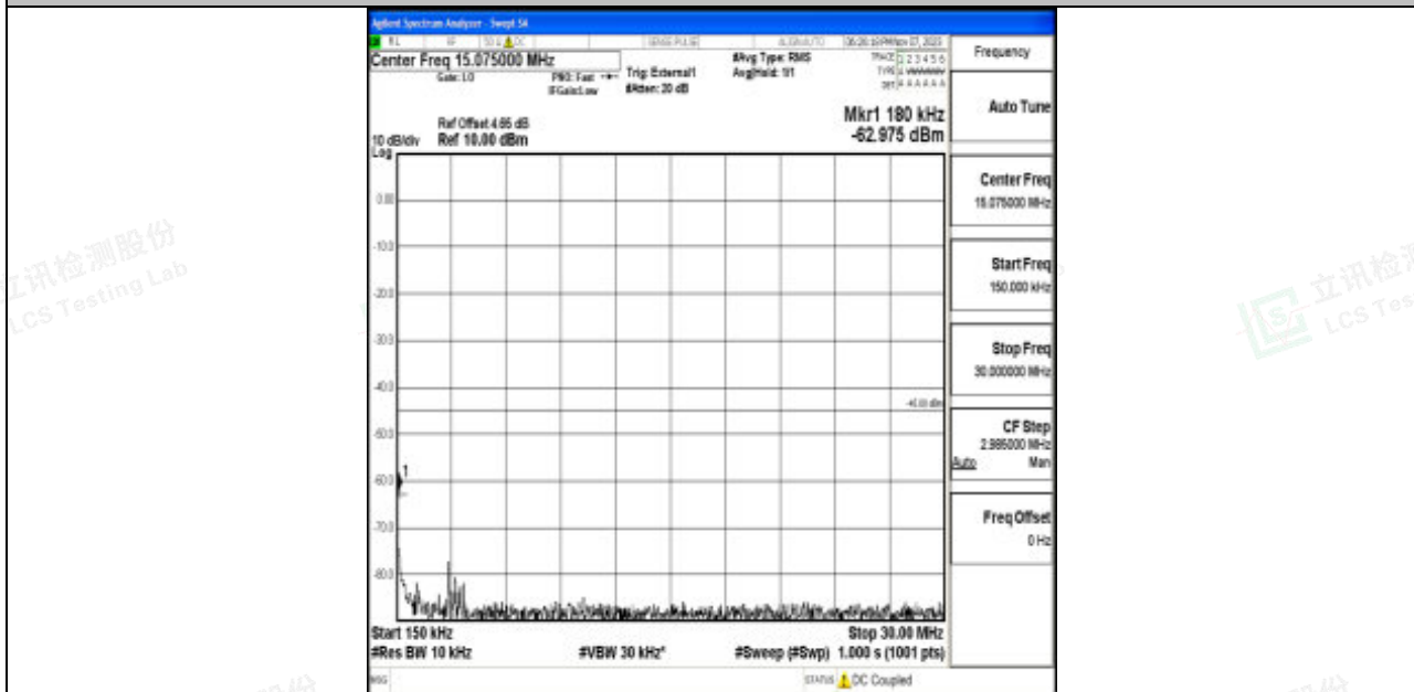
Band41_10MHz_64QAM_41540_1RB#0_0.15~30_0.15~30
