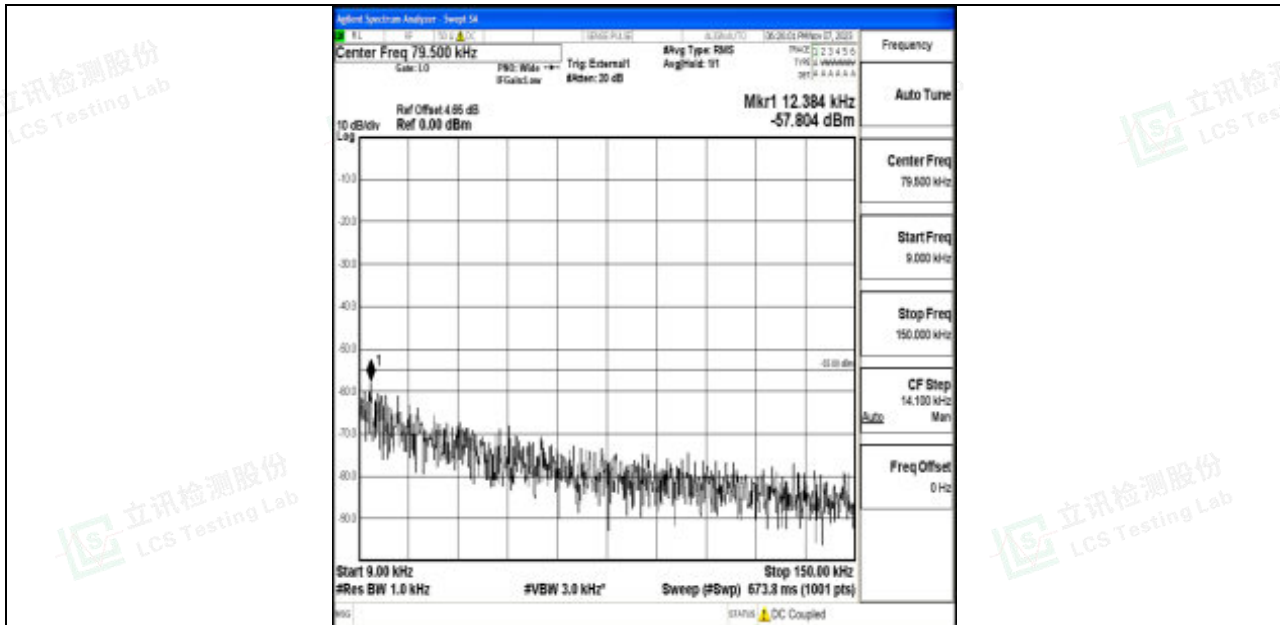
Band41_10MHz_64QAM_41540_1RB#0_0.009~0.15_0.009~0.15
