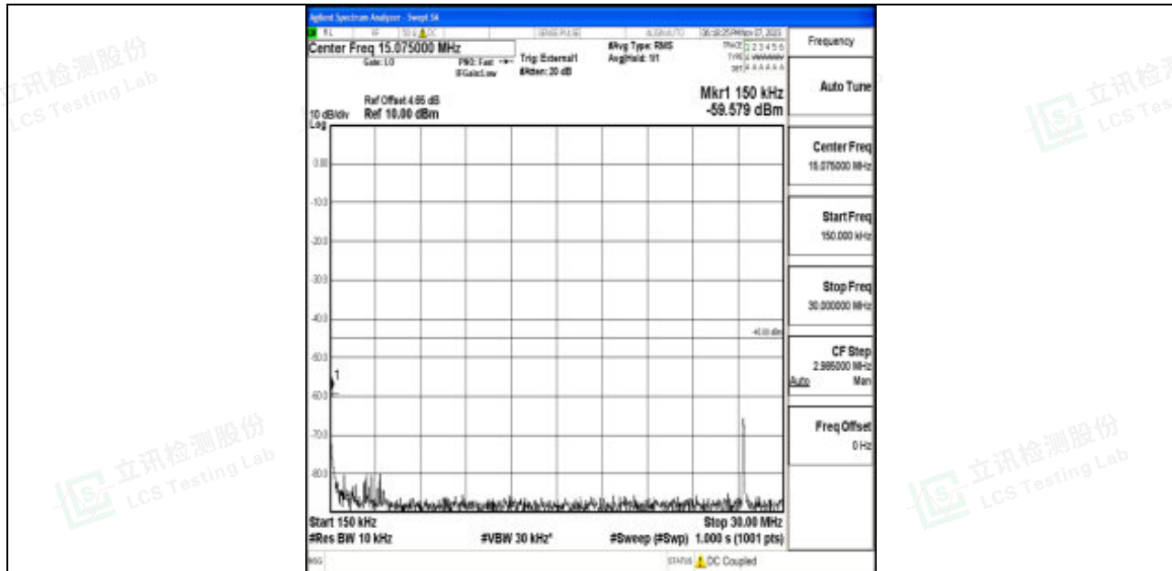
Band41_10MHz_QPSK_40620_1RB#0_0.15~30_0.15~30
