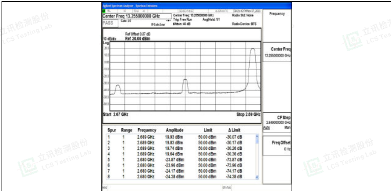
Band41_20MHz_64QAM_41490_1RB#99
