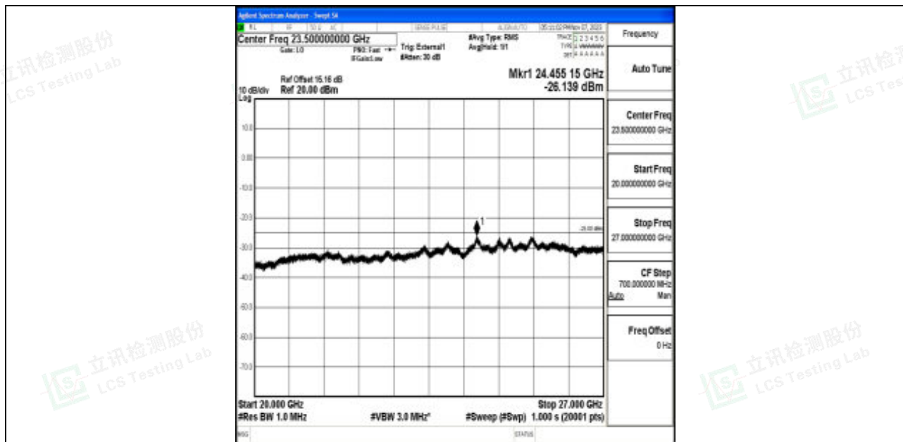
Band41_5MHz_16QAM_41565_1RB#0_20000~27000_20000~27000
