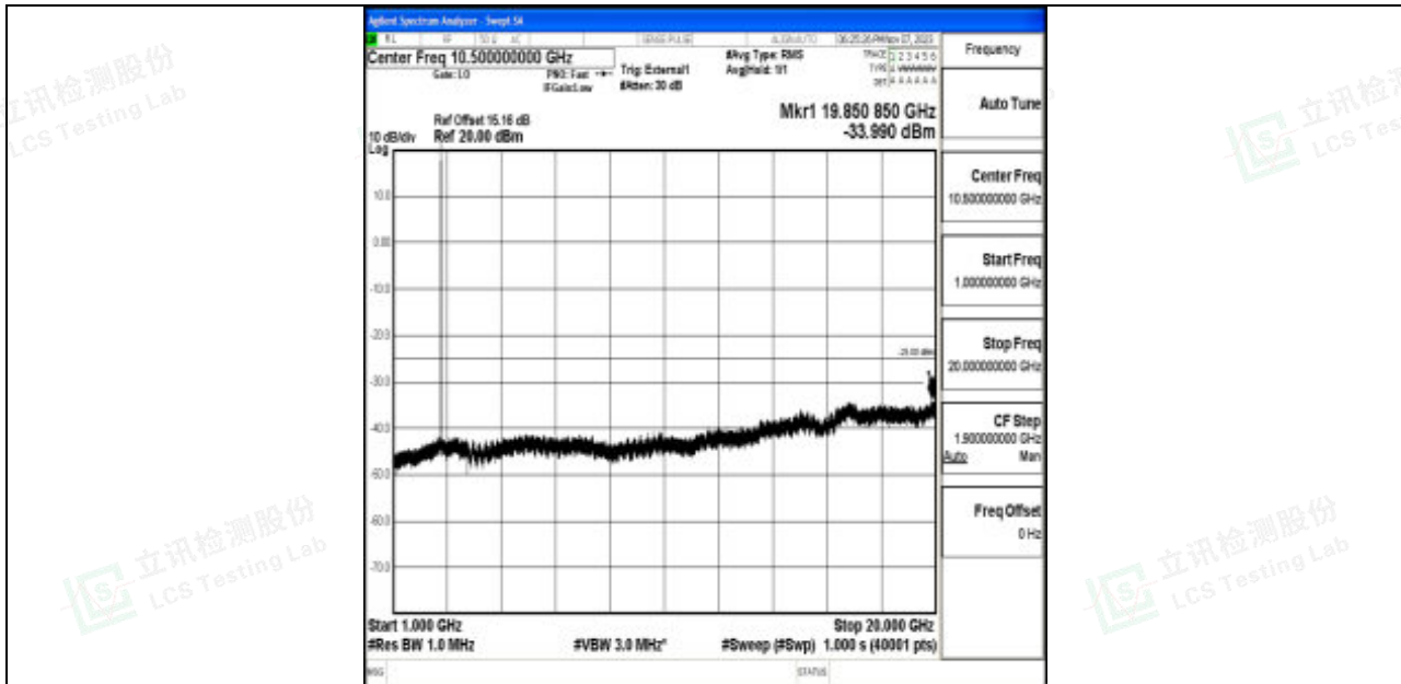
Band41_10MHz_16QAM_41540_1RB#0_1000~20000_1000~20000
