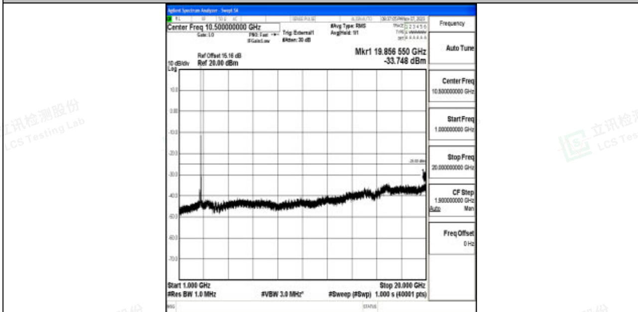
Band41_20MHz_QPSK_41490_1RB#0_1000~20000_1000~20000
