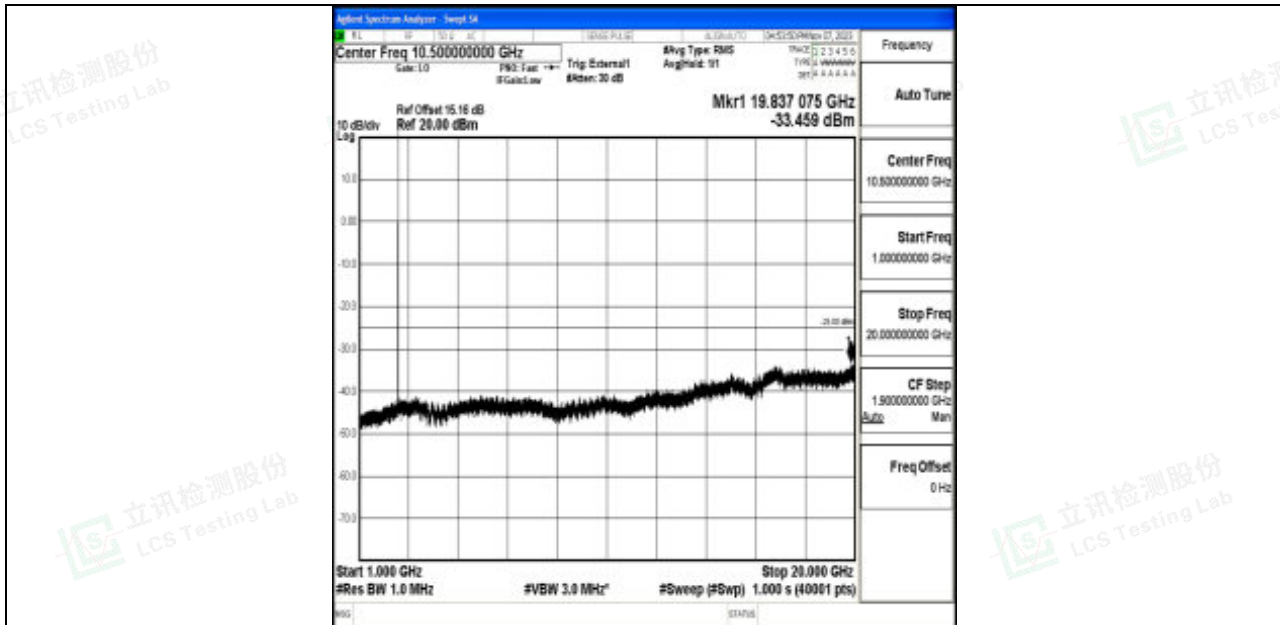
Band41_5MHz_QPSK_39675_1RB#0_1000~20000_1000~20000
