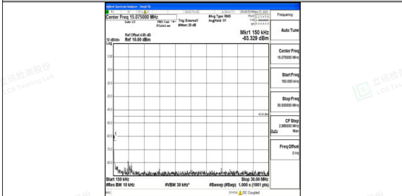
Band41_5MHz_16QAM_41565_1RB#0_0.15~30_0.15~30
