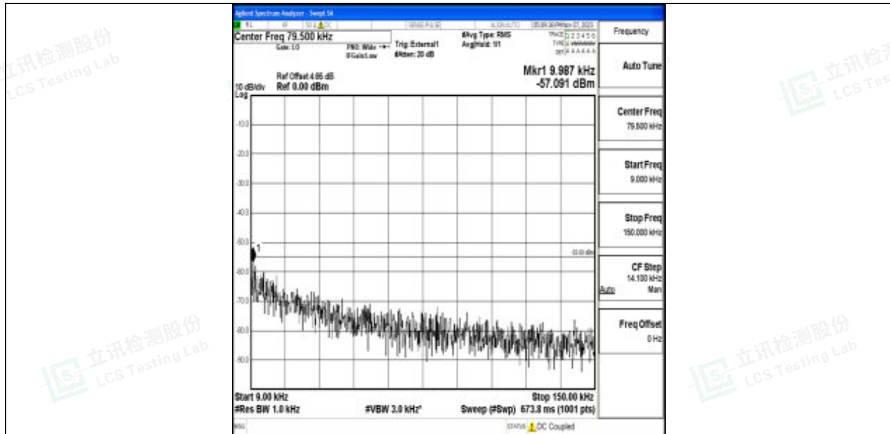
Band41_5MHz_16QAM_41565_1RB#0_0.009~0.15_0.009~0.15
