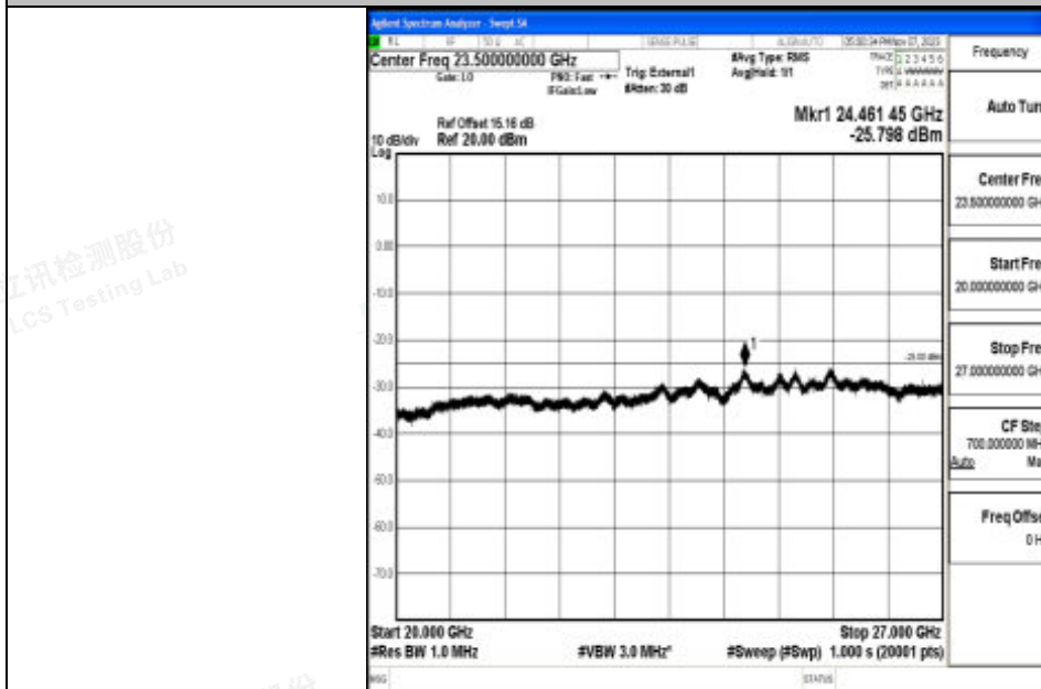
Band41_5MHz_16QAM_40620_1RB#0_20000~27000_20000~27000
