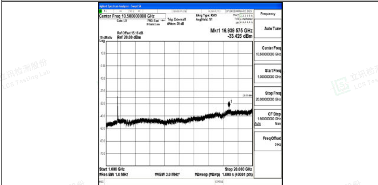
Band41_15MHz_16QAM_39725_1RB#0_1000~20000_1000~20000
