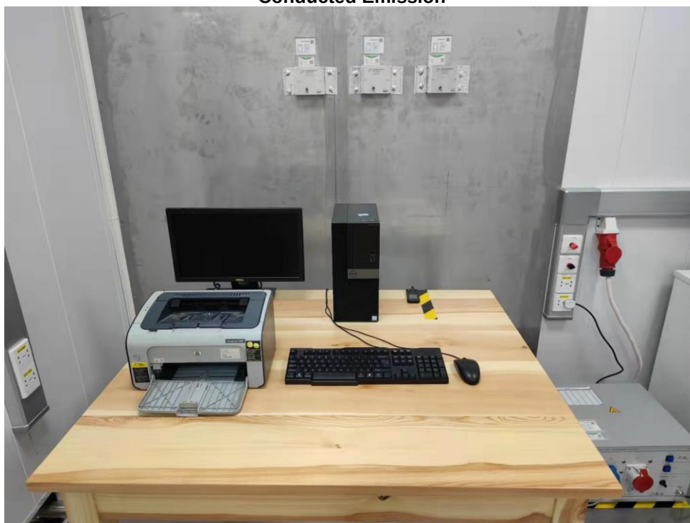
Conducted Emission
