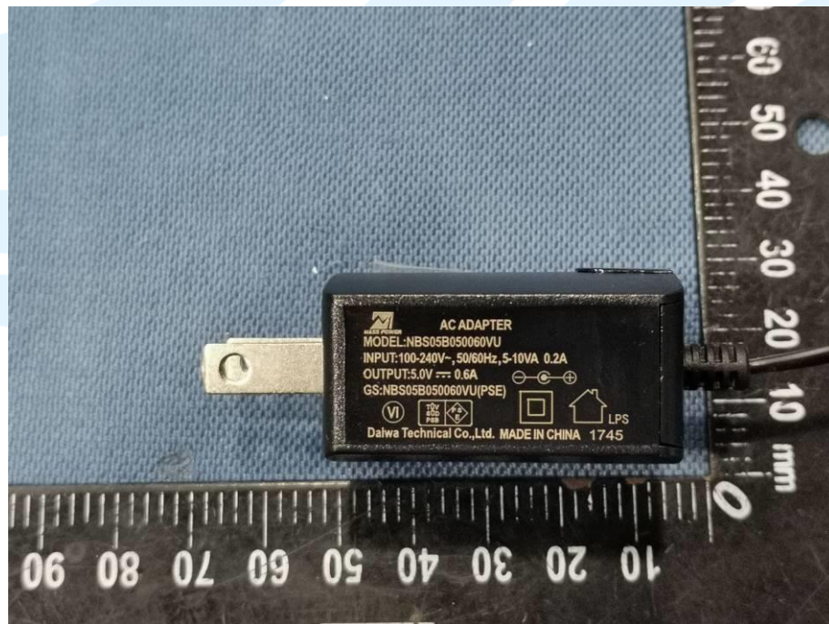
EUT Photo(Adapter 2: NBS05B050060VU)
