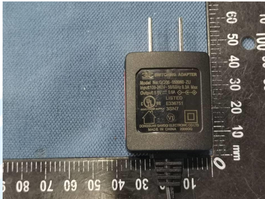
EUT Photo(Adapter 1: GQ06-050060-ZU)
