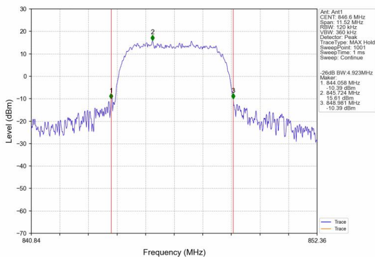
Band5 HSDPA HCH 846.6MHz Subtest 1 NTNv
