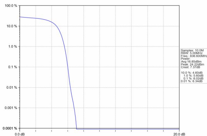
Band5 HSDPA MCH 836.6MHz Subtest 1 NTN
