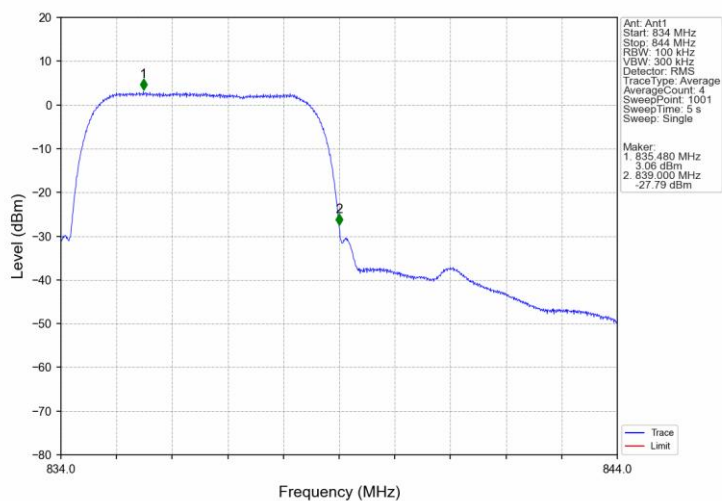
Band5 HSUPA MCH 836.6MHz Subtest 1 NTN
