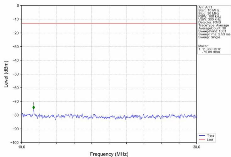
Band5 HSUPA HCH 846.6MHz Subtest 1 NTNv
