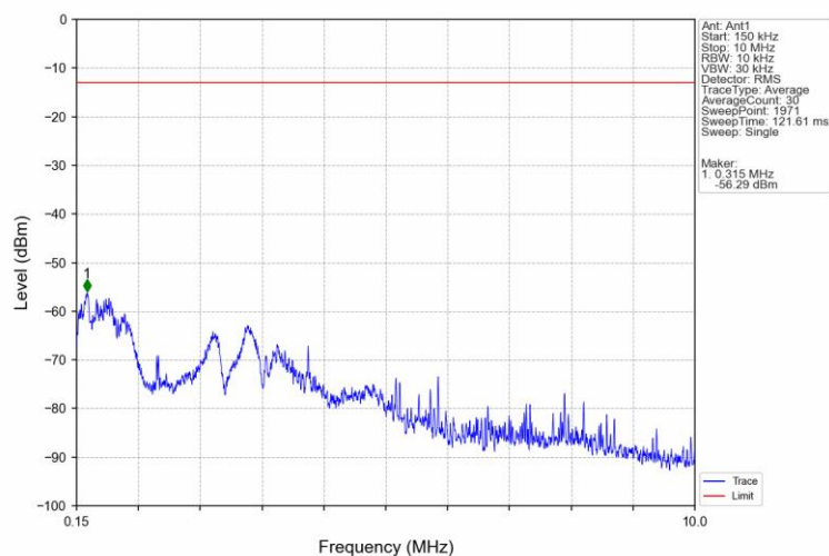
Band5 HSUPA HCH 846.6MHz Subtest 1 NTNv
