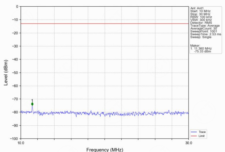
Band5_HSUPA_LCH_826.4MHz_Subtest 1_NTNV
