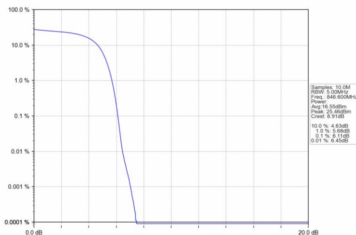
Band5 HSDPA HCH 846.6MHz Subtest 1 NTN
