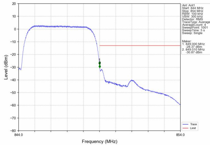
Band5 HSUPA HCH 846.6MHz Subtest 1 NTN
