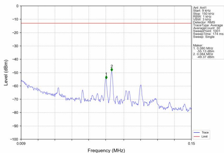
Band5 HSUPA MCH 836.6MHz Subtest 1 NTNv
