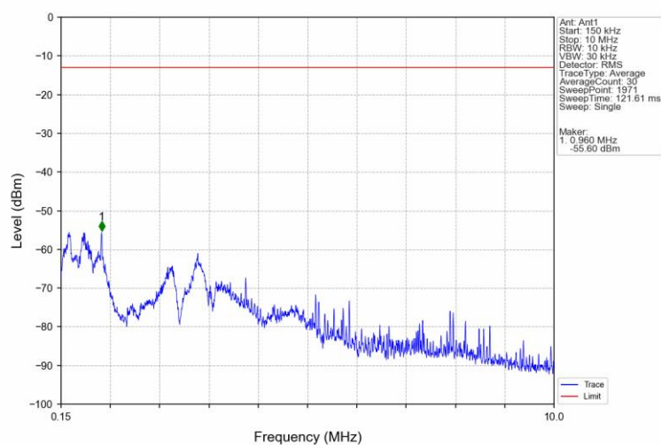
Band5_HSDPA_LCH_826.4MHz_Subtest 1_NTNV
