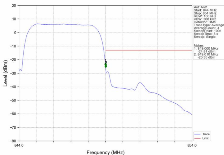
Band5_RMC_HCH_846.6MHz_12.2kbps_RMC_NTNV
