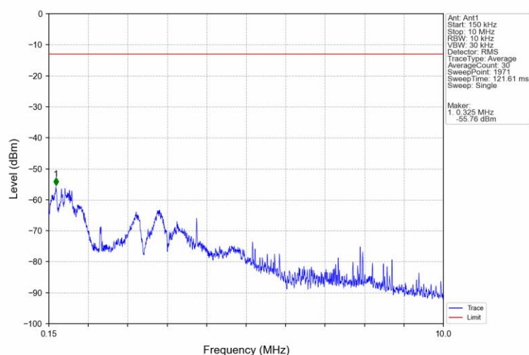
Band5 HSUPA MCH 836.6MHz Subtest 1 NTNv
