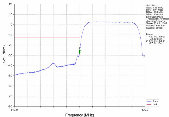
Band5_HSUPA_LCH_826.4MHz_Subtest 1_NTNV
