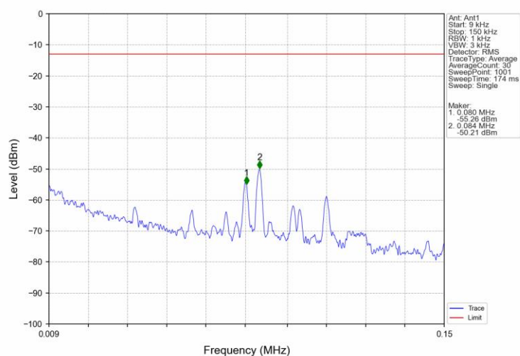
Band5_HSDPA_HCH_846.6MHz_Subtest 1_NTNV
