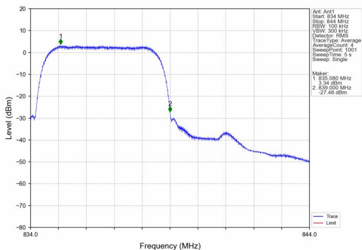
Band5 HSDPA MCH 836.6MHz Subtest 1 NTN
