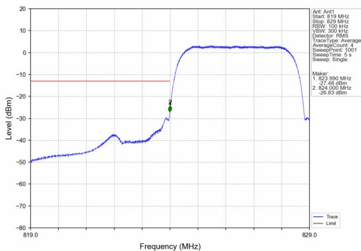
Band5_HSDPA_LCH_826.4MHz_Subtest 1_NTNV
