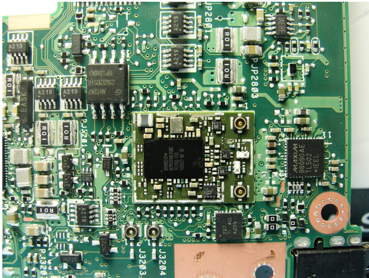
EUT: WLAN module (Brand Name: AzureWave / Model Name: AW-CM195NF)
