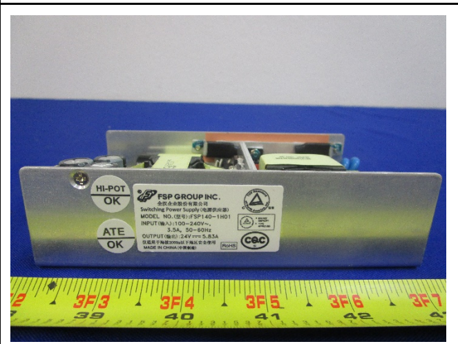
PCBA3 Label View
