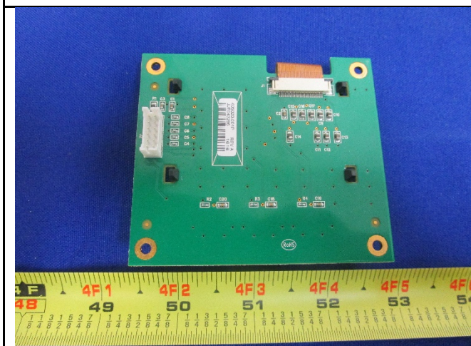
Display Board Bottom View 1
