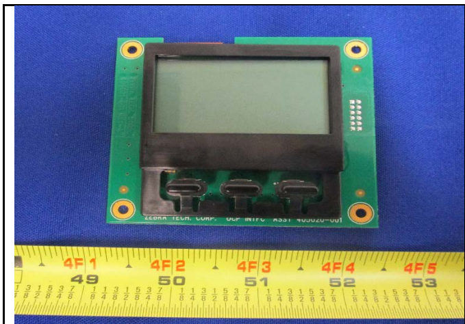
Display Board Top View 1
