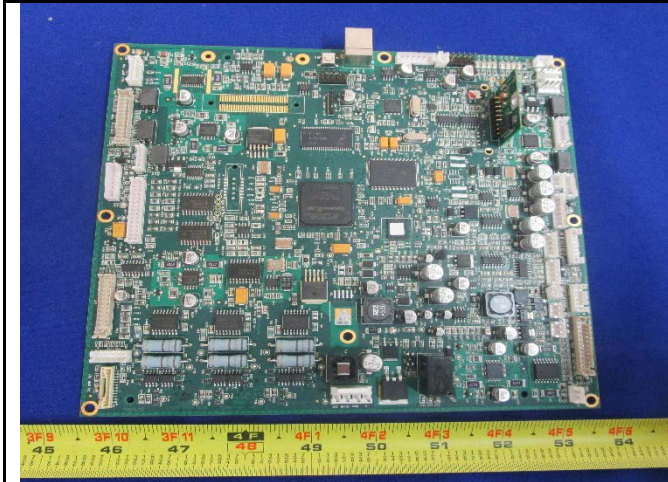
EUT-Main PCBA Component View
