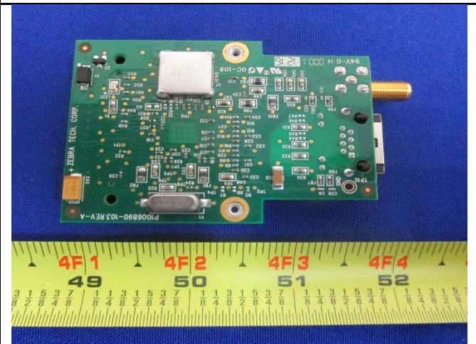
WIFI Radio Board Bottom View
