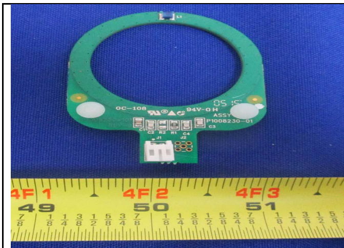
Ribbon RFID1 Antenna Top View
