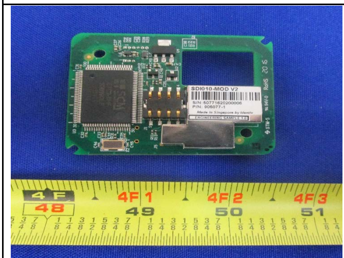
Contactless RFID Board Top View
