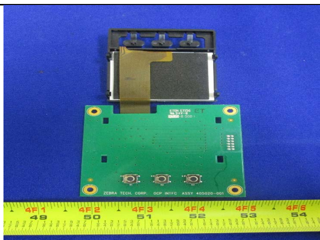
Display Board Bottom View 2
