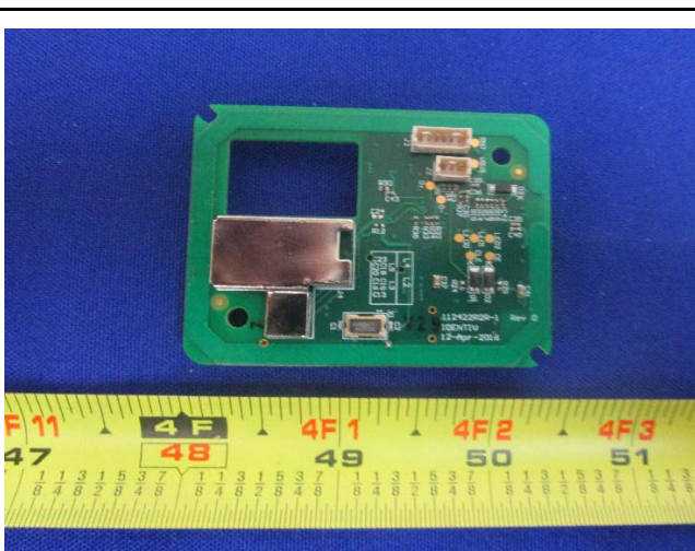
Contactless RFID Board Bottom View
