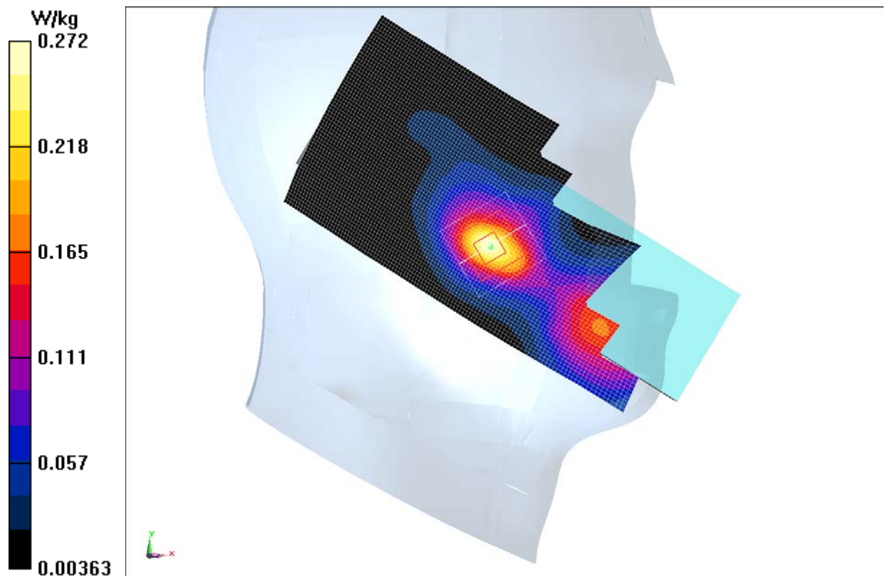
Fig.3 1900 MHz
