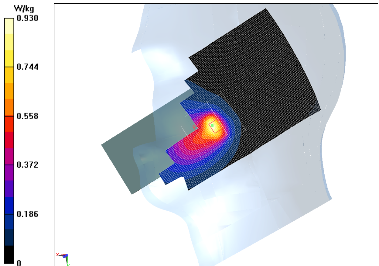
Fig.1 850MHz
