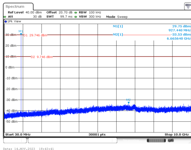
CSE Plot on 927.25 MHz between 30MHz ~ 10 GHz
