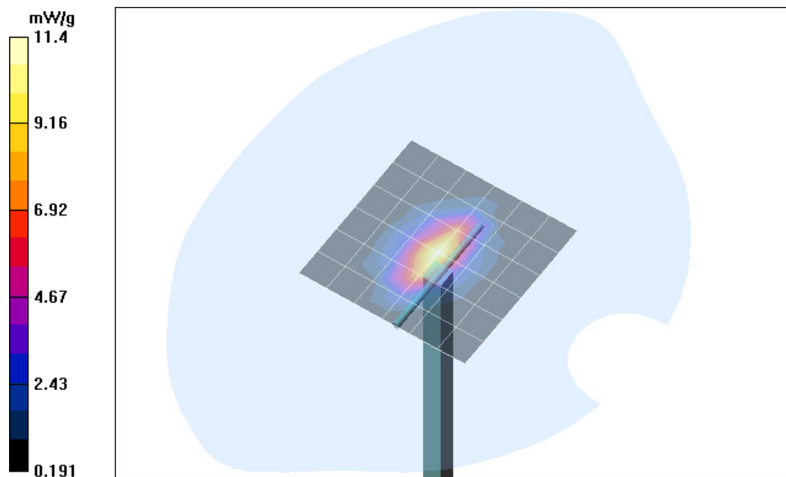
Fig. 11: Validation measurement 1900 MHz body (June 11, 2004), coarse grid. Ambient Temperature: 21.8° C, Liquid Temperature: 20.6° C.
