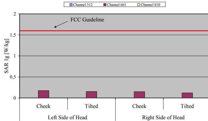
Fig. 8: The measured head phantom SAR values for the Alcatel One Touch 565 for PCS 1900 in comparison to the FCC exposure limit.
