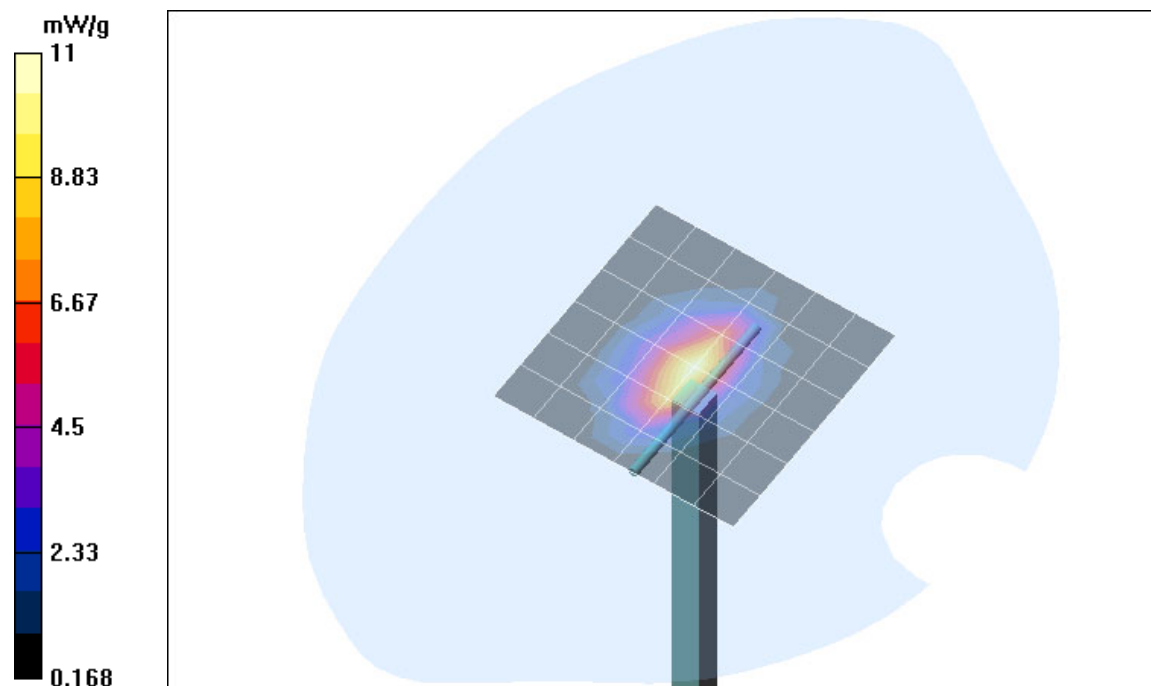
Fig. 10: Validation measurement 1900 MHz Head (June 09, 2004), coarse grid. Ambient Temperature: 22.0° C, Liquid Temperature: 21.0 C.
