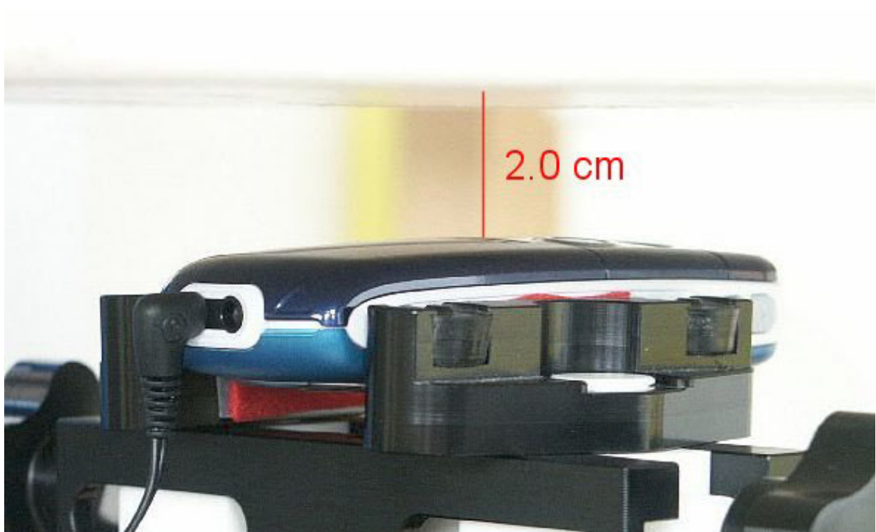
Fig. 21: Body worn configuration, GSM mode (1 TX slot) with headset, antenna towards the phantom.
