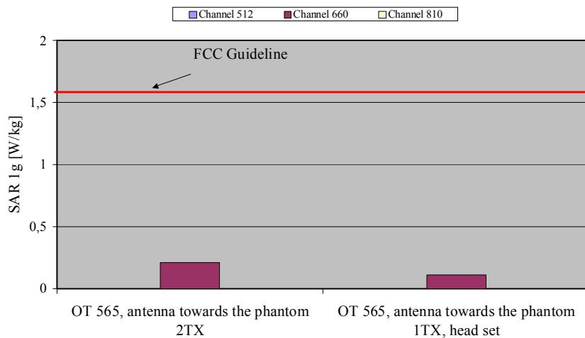
Fig. 9: The measured SAR values in body-worn configuration for the Alcatel One Touch 565 for PCS 1900 (1 TX and 2 TX slots, gap = 2.0 cm) in comparison to the FCC exposure limit.
