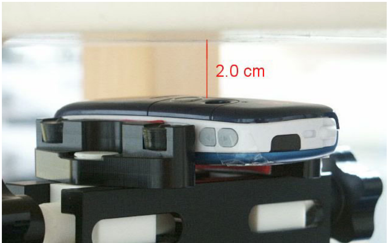
Fig. 20: Body worn configuration, GPRS mode (2 TX slots), antenna towards the phantom.
