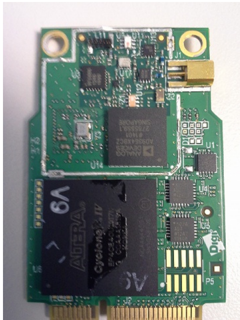
Internal Top
