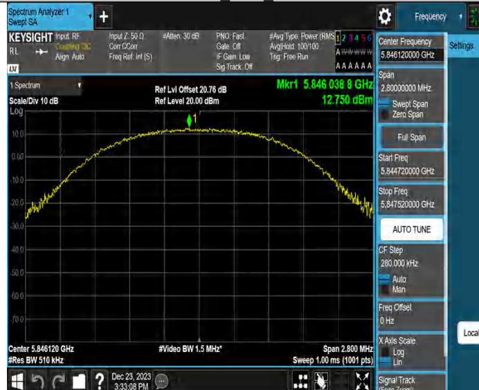
1.4MCA_Ant2_5846.12
