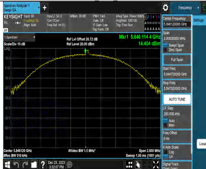
1.4MCA_Ant2_5846.12
