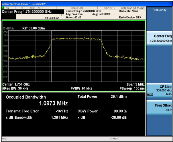
Band4-1.4MHz-QPSK-20393-6RB#0-PASS
