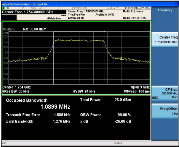
Band4-1.4MHz-16QAM-20393-6RB#0-PASS
