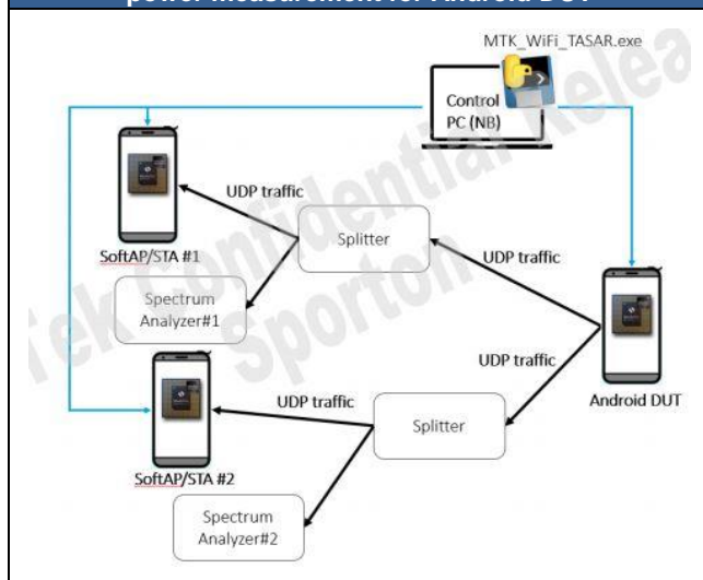
Figure 6-1 General setup for TA-SAR conducted power measurement for Android DUT
