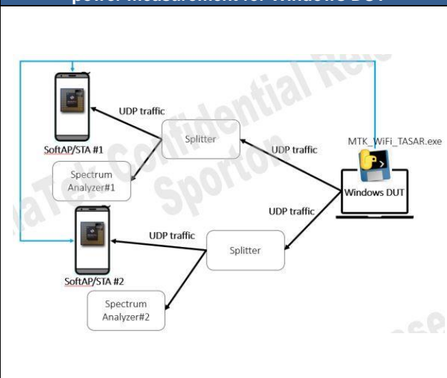
Figure 6-2 General setup for TA-SAR conducted power measurement for Windows DUT
