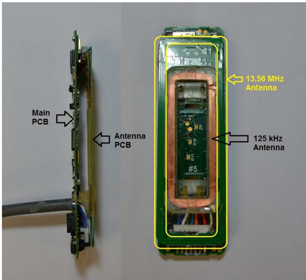
T15 Multi Tech - 125 kHz & 13.56 MHz Antennas and Main PCB
