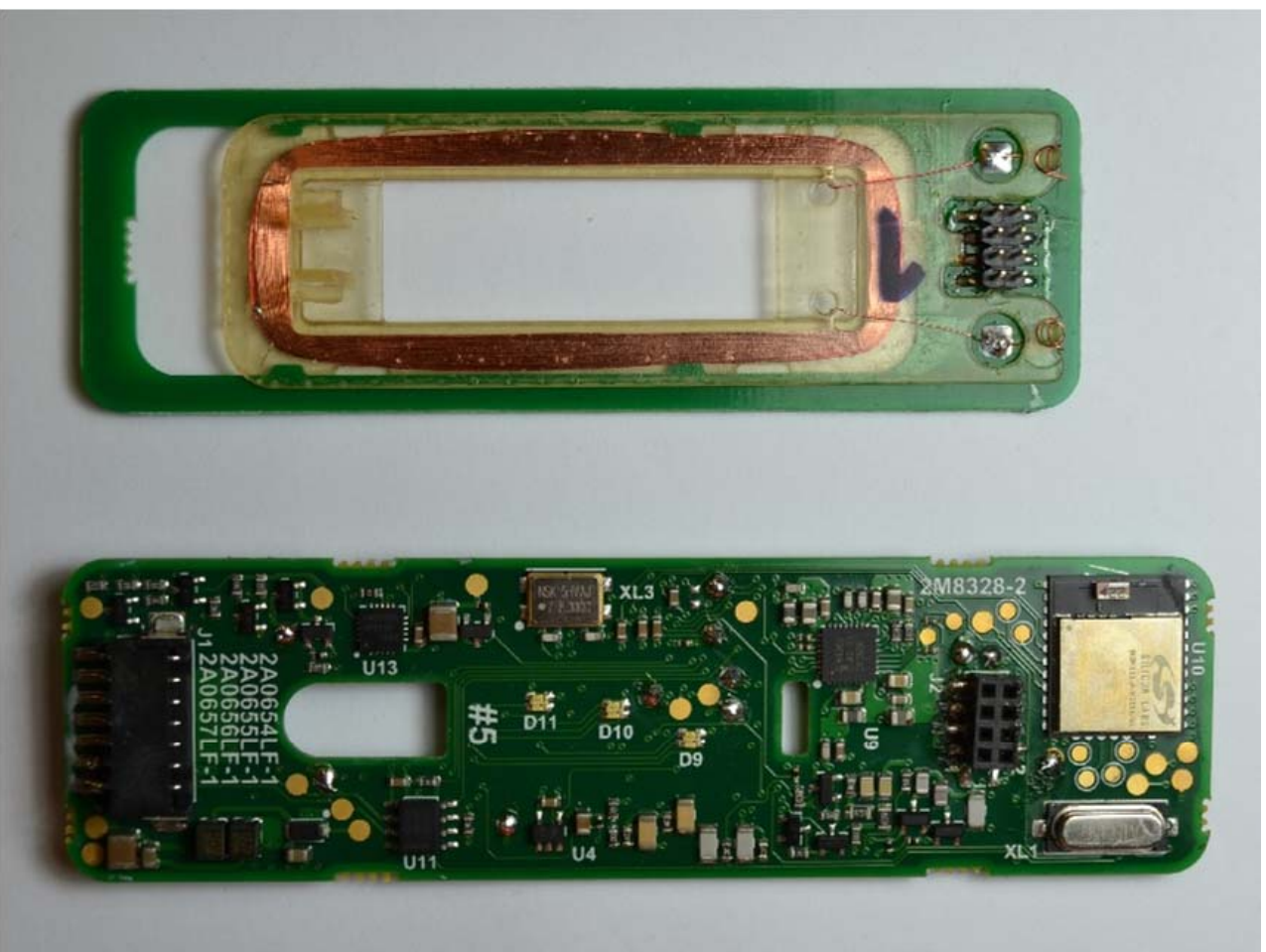
T15 Multi Tech - Main and Antenna PCB (Front)
