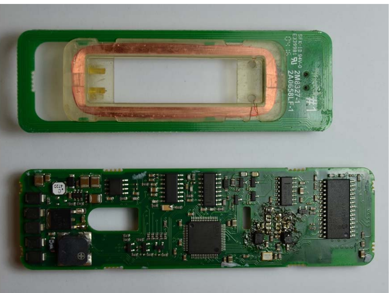
T15 Multi Tech - Main and Antenna PCB (Rear)
