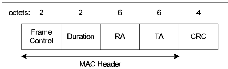
Figure 9.21: CTS Frame
