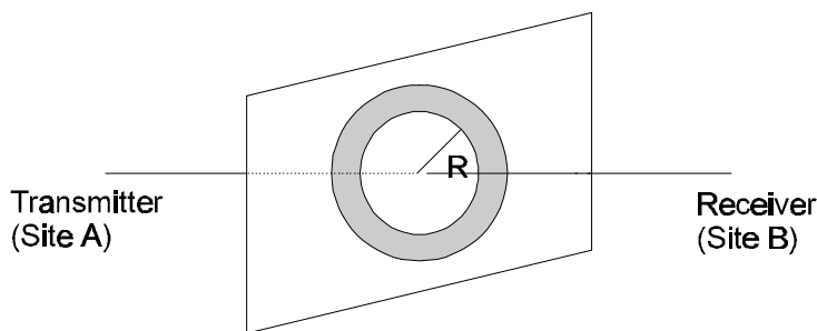
Figure 9.12: Fresnel Zone
