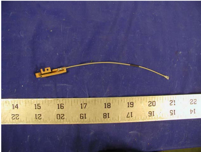
BM1 Antenna Right Side
