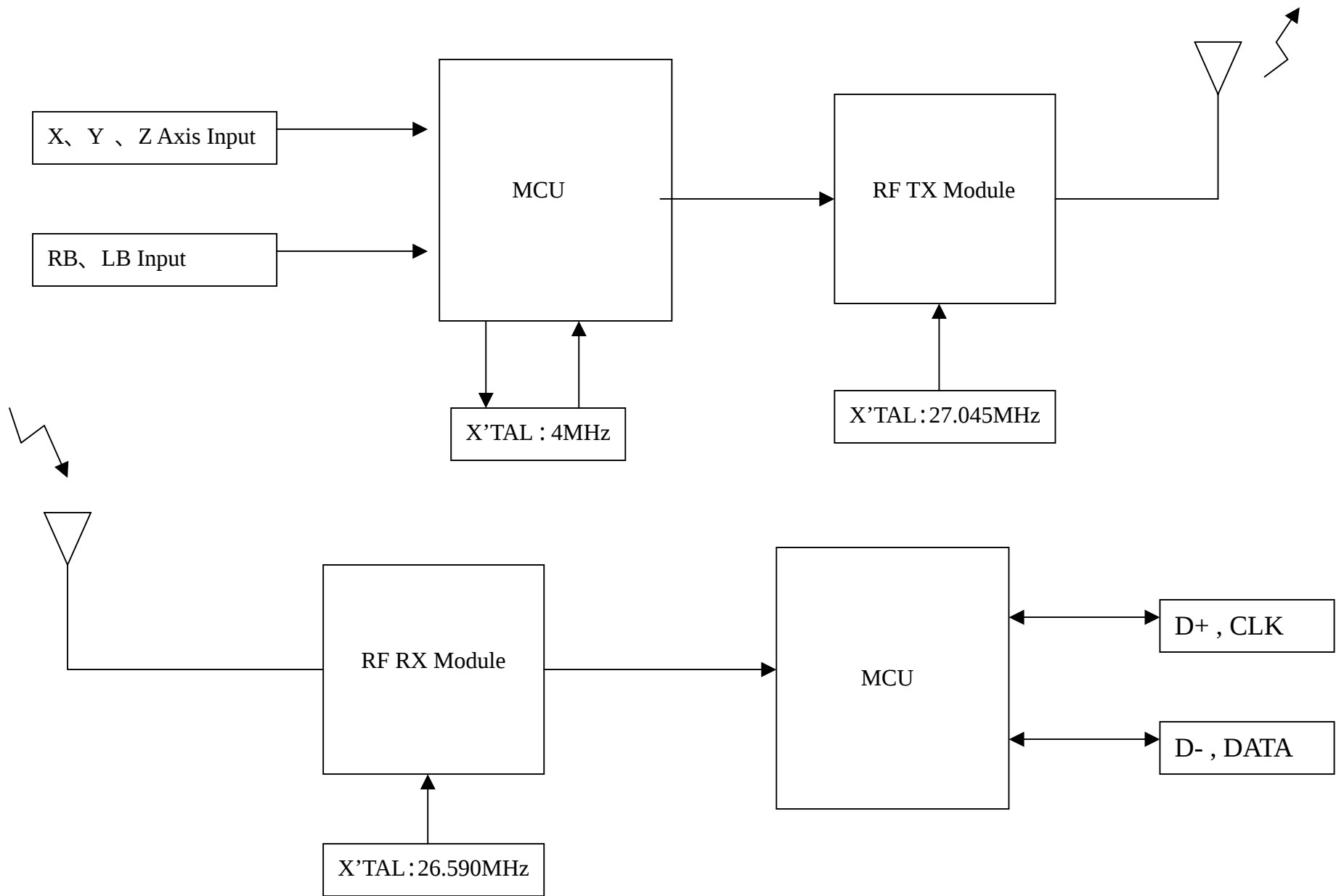
RF MOUSE BLOCK DIAGRAM
