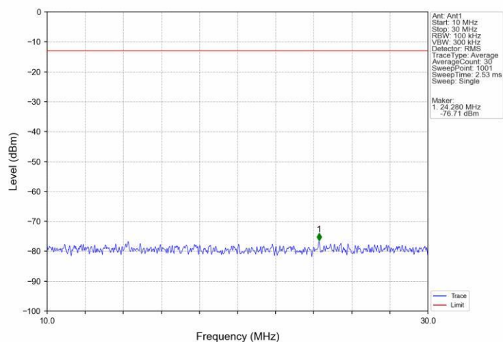
Band71 15MHz 16QAM HCH 690.5MHz RB 1 0 NTV
