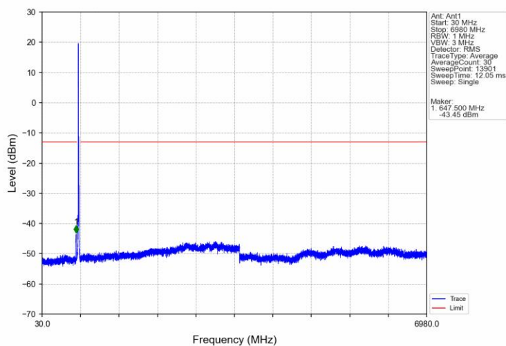
Band71 15MHz 16QAM HCH 690.5MHz RB 1 0 NTV
