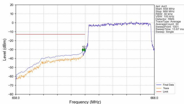
Band71_5MHz_16QAM_LCH_665.5MHz_RB_25_0_NTV
