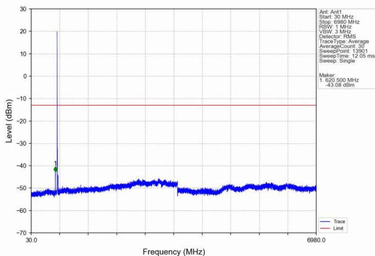
Band71_5MHz_16QAM_LCH_665.5MHz_RB_25_0_NTV
