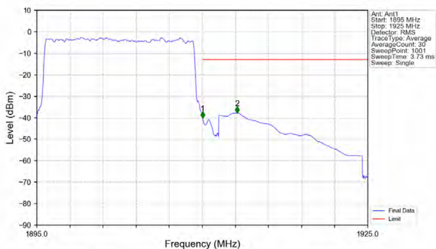
Band2_15MHz_QPSK_HCH_1902.5MHz_RB_75_0_NTNV
