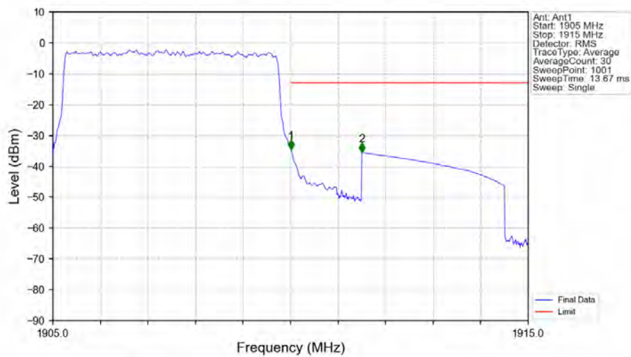
Band2_5MHz_QPSK_HCH_1907.5MHz_RB 25_0_NTNV
