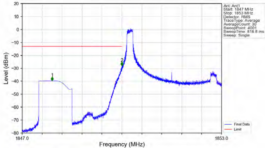
Band2_3MHz_16QAM_LCH_1851.5MHz_RB_1_0_NTNV
