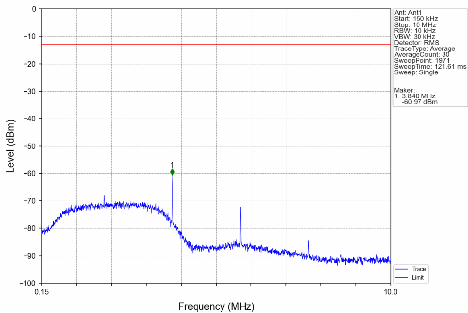
Band5_RMC_HCH_846.6MHz_12.2kbps RMC_NTNV
