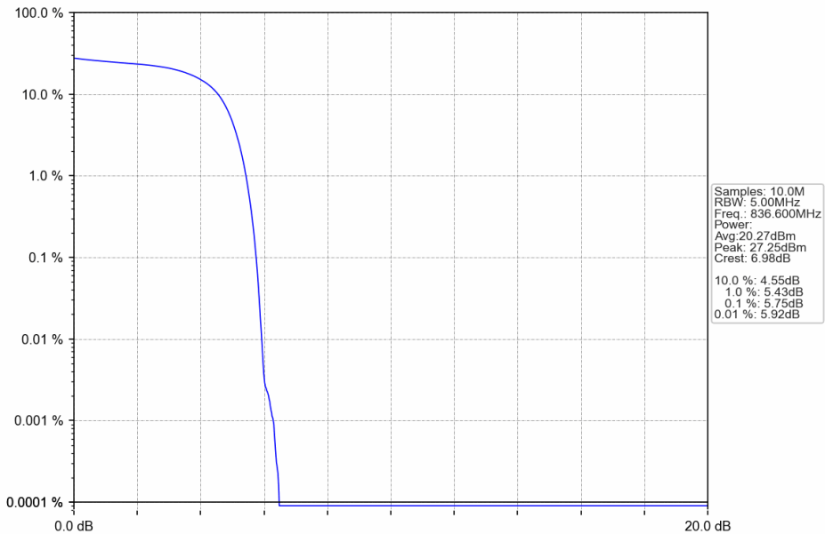
Band5_HSDPA_MCH_836.6MHz_Subtest 1_NTNV
