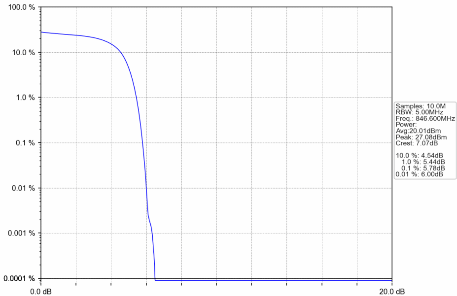
Band5_HSDPA_HCH_846.6MHz_Subtest 1_NTNV
