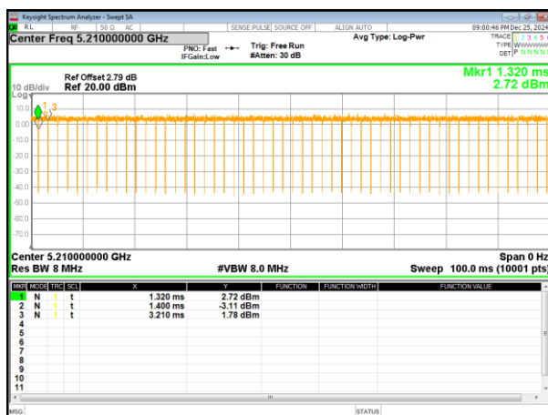
(802.11ac80) plot
