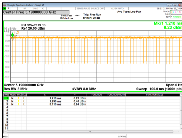
(802.11 n40) plot
