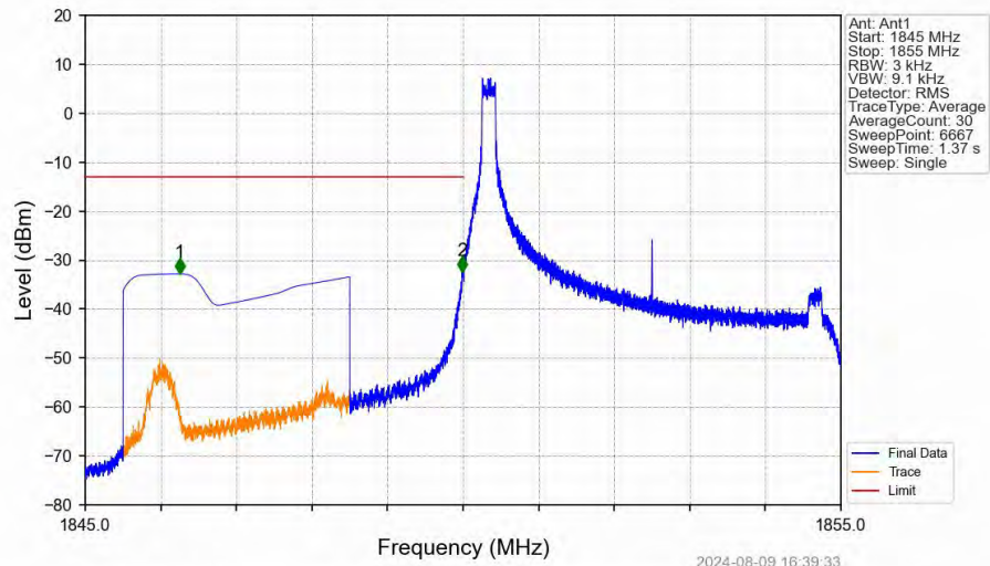
Band25_5MHz_16QAM_LCH_1852.5MHz_RB_1_0_NTNV
