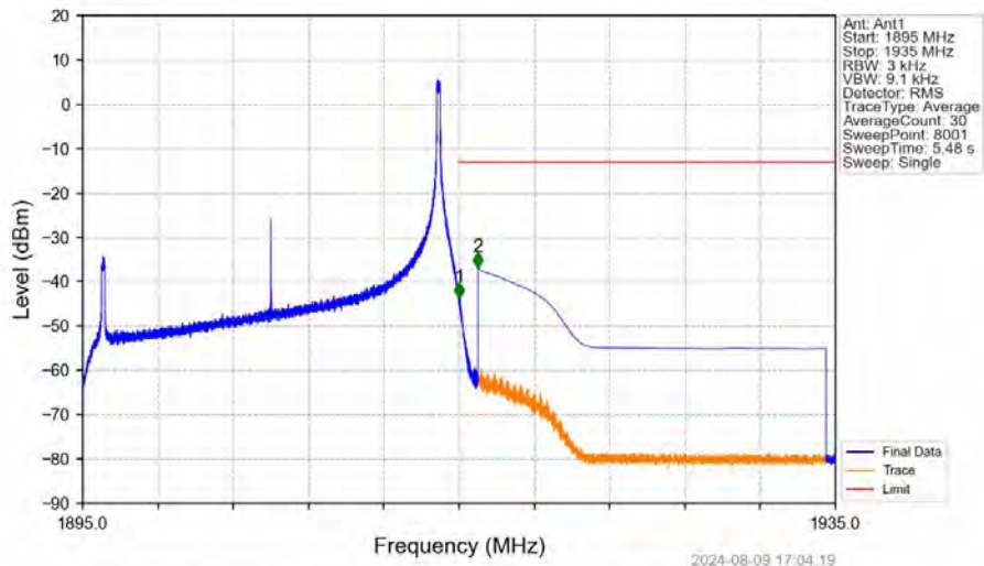
Band25_20MHz_16QAM_HCH_1905MHz_RB_1_99_NTNV
