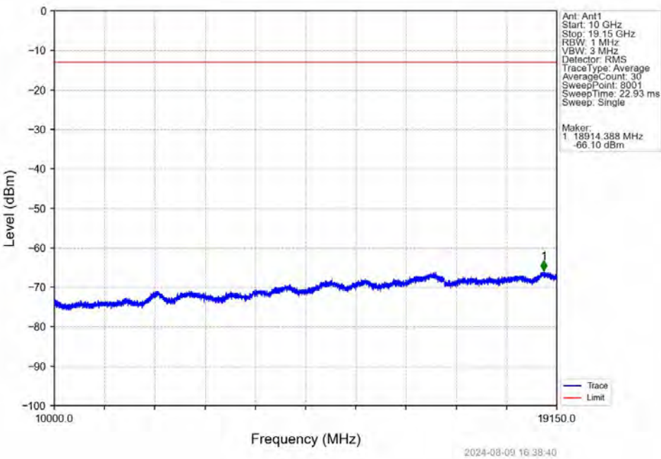
Band25_5MHz_QPSK_LCH_1852.5MHz_RB_25_0_NTNV
