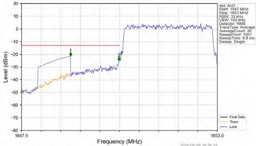
Band25_3MHz_16QAM_LCH_1851.5MHz_RB_15_0_NTNV
