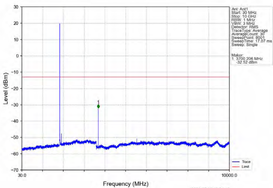
Band25_3MHz_16QAM_LCH_1851.5MHz_RB_1_0_NTNV
