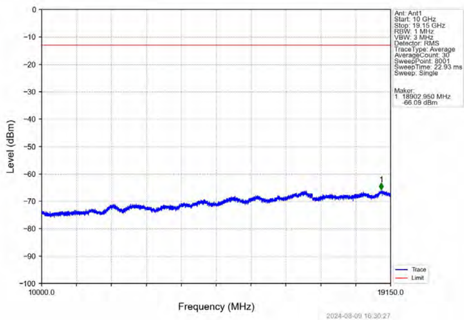
Band25_1.4MHz_QPSK_MCH_1882.5MHz_RB_1_0_NTNV
