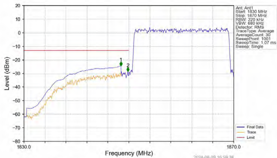
Band25_20MHz_16QAM_LCH_1860MHz_RB_100_0_NTNV
