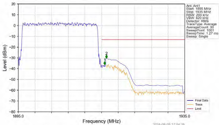
Band25_20MHz_16QAM_HCH_1905MHz_RB_100_0_NTNV
