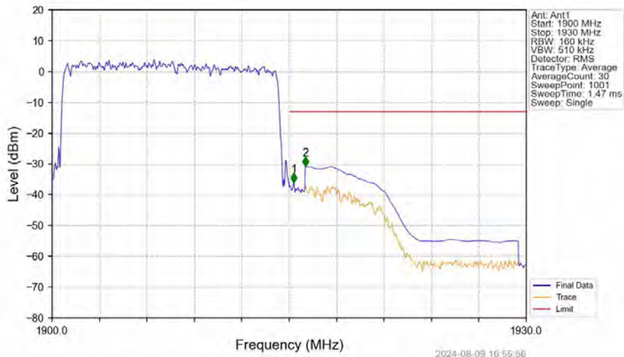
Band25_15MHz_16QAM_HCH_1907.5MHz_RB_75_0_NTNV
