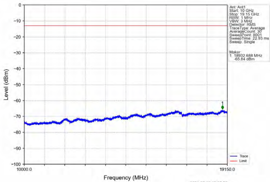
Band25_5MHz_16QAM_LCH_1852.5MHz_RB_25_0_NTNV
