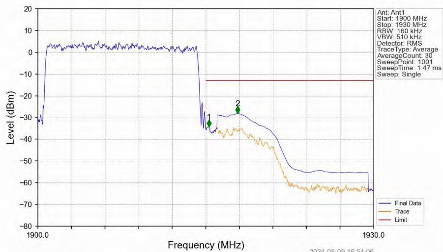
Band25_15MHz_QPSK_HCH_1907.5MHz_RB_75_0_NTNV
