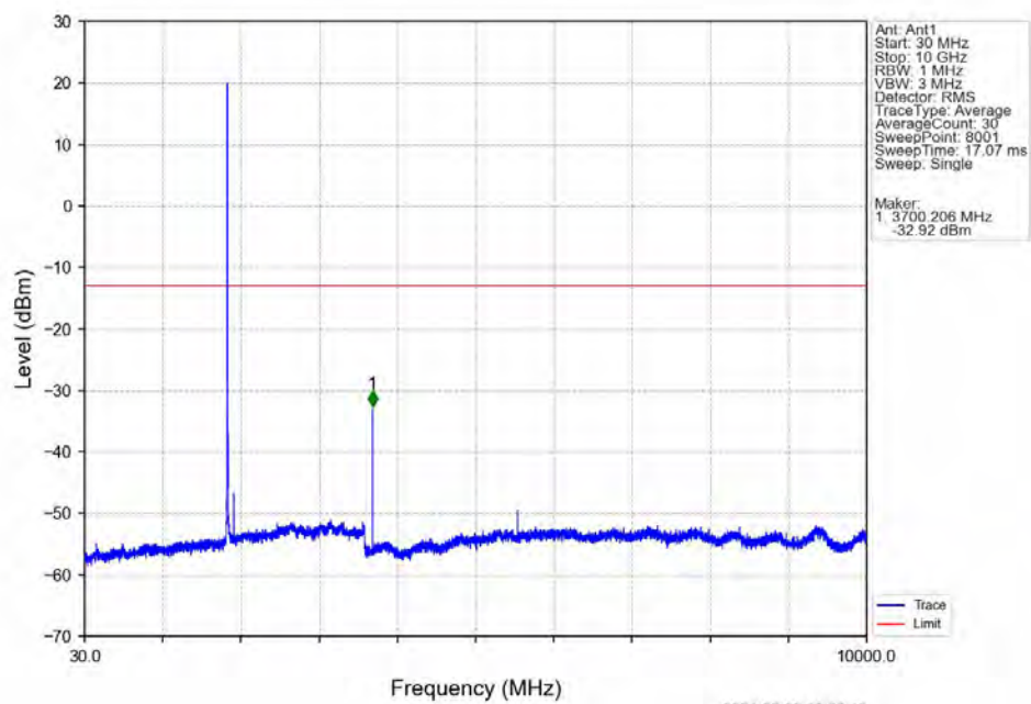
Band25_5MHz_16QAM_LCH_1852.5MHz_RB_1_0_NTNV
