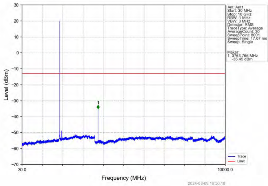
Band25_1.4MHz_QPSK_MCH_1882.5MHz_RB_1_0_NTNV
