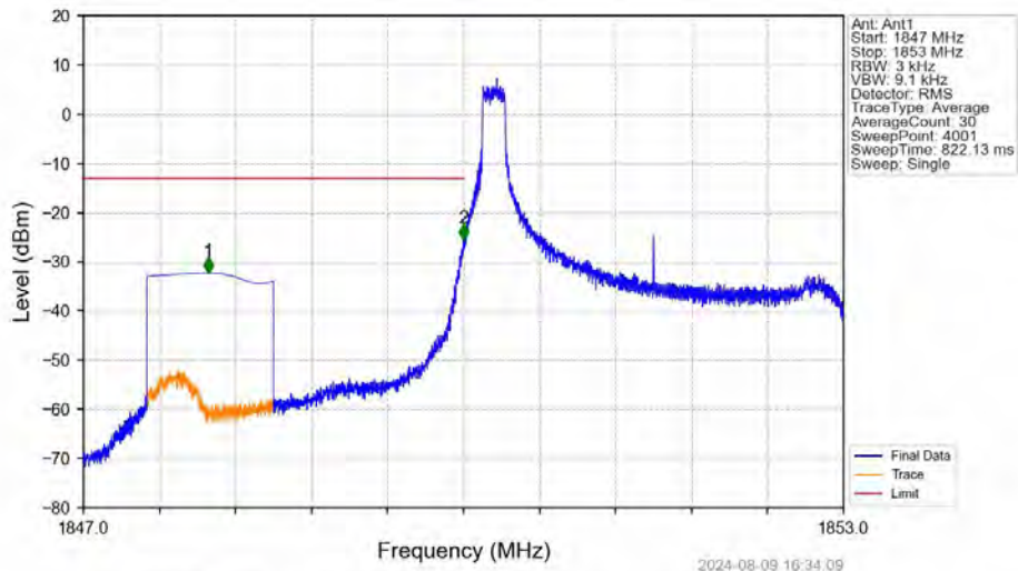
Band25_3MHz_16QAM_LCH_1851.5MHz_RB_1_0_NTNV
