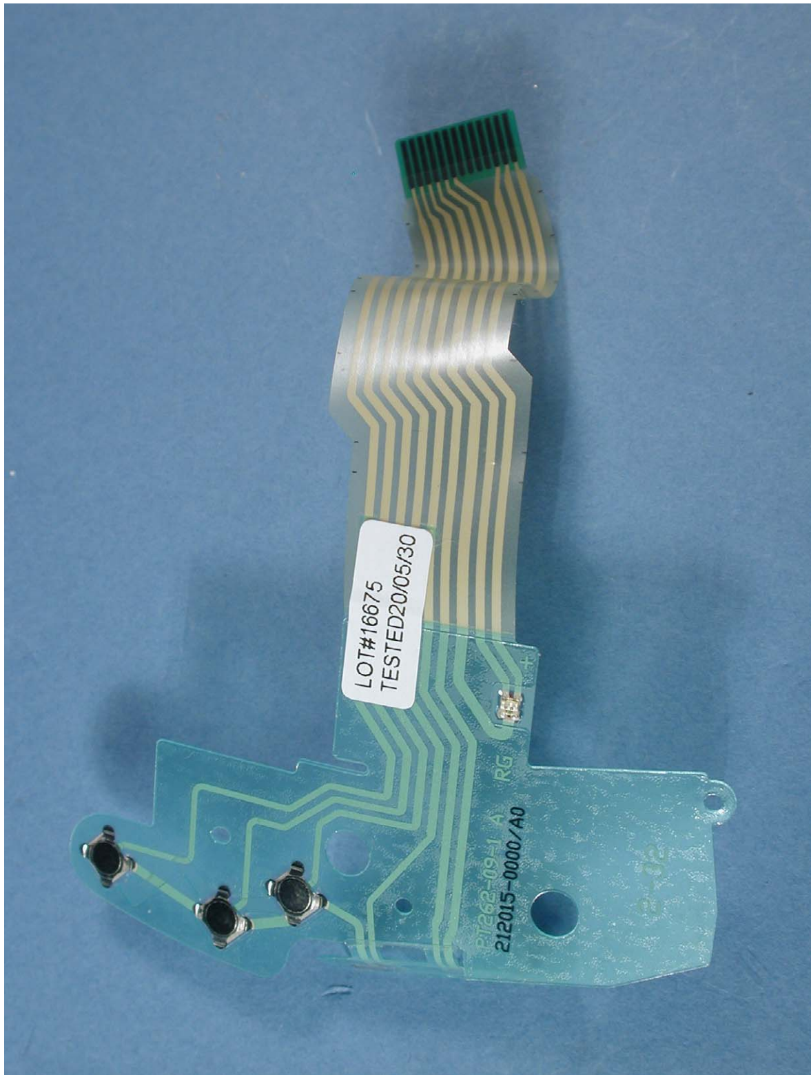
Photograph 12: Membrane PCB of M-RAZ105
