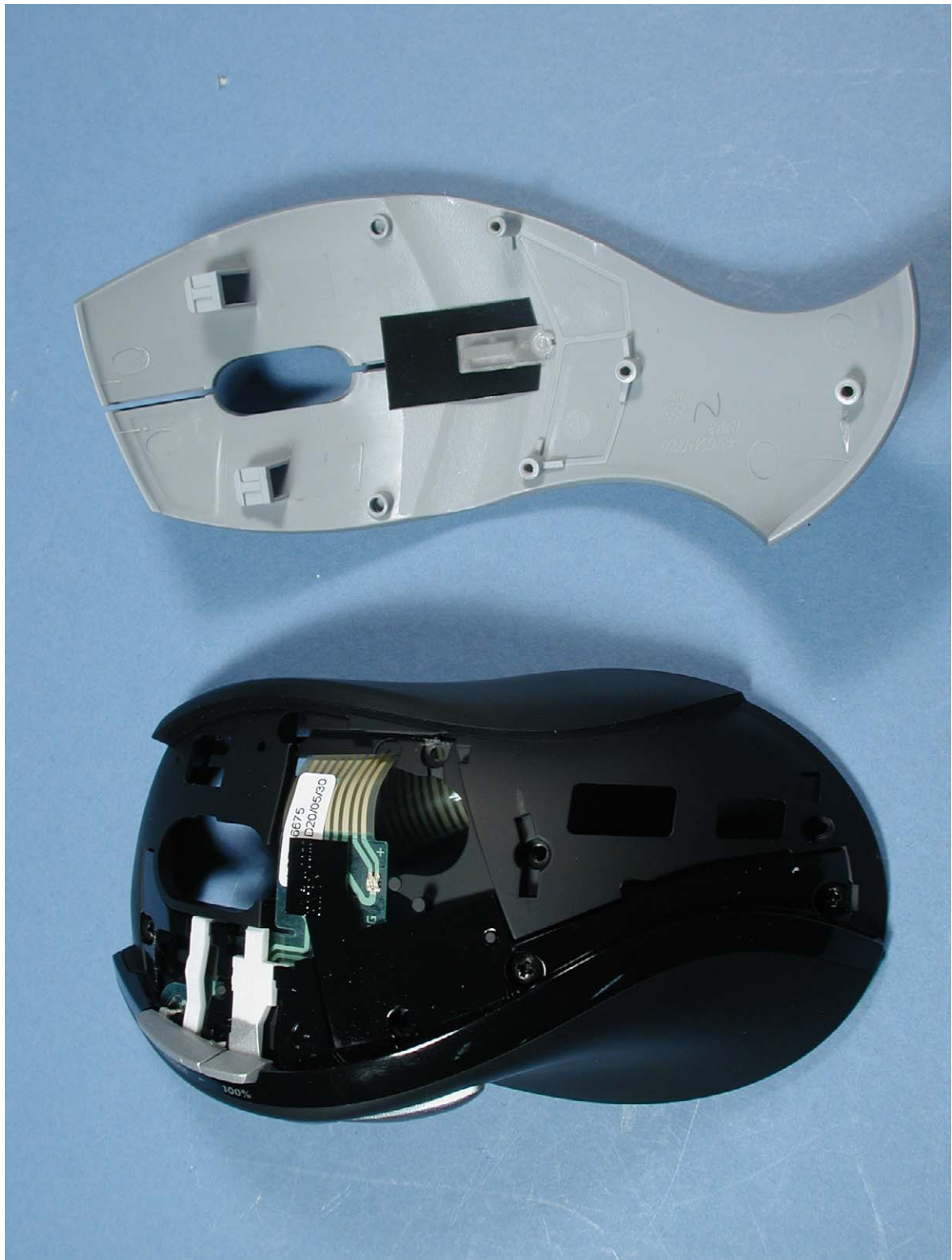
Photograph 10: Top view of M-RAZ105 without cover
