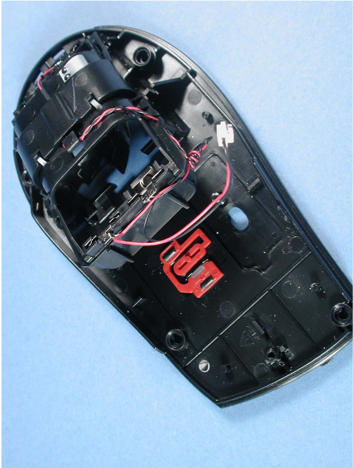
Photograph 13: Base of M-RAZ105 including battery compartment
