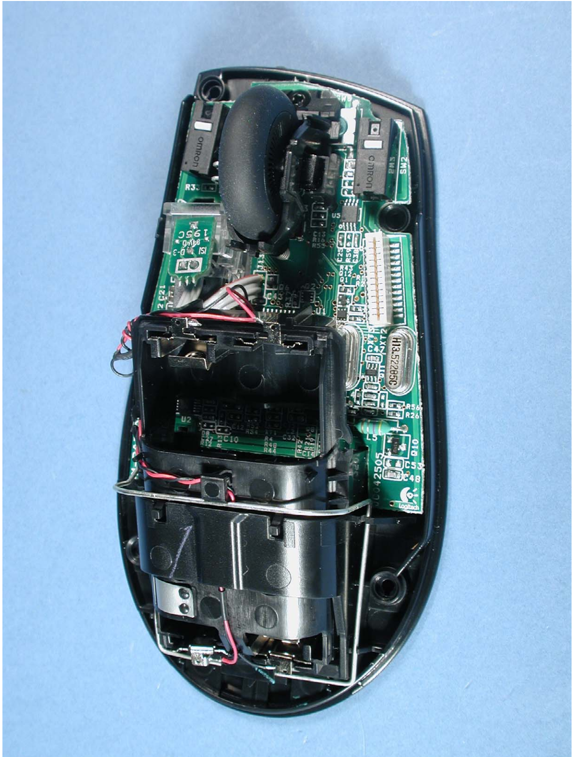
Photograph 6: Inside view of M-RAZ105
