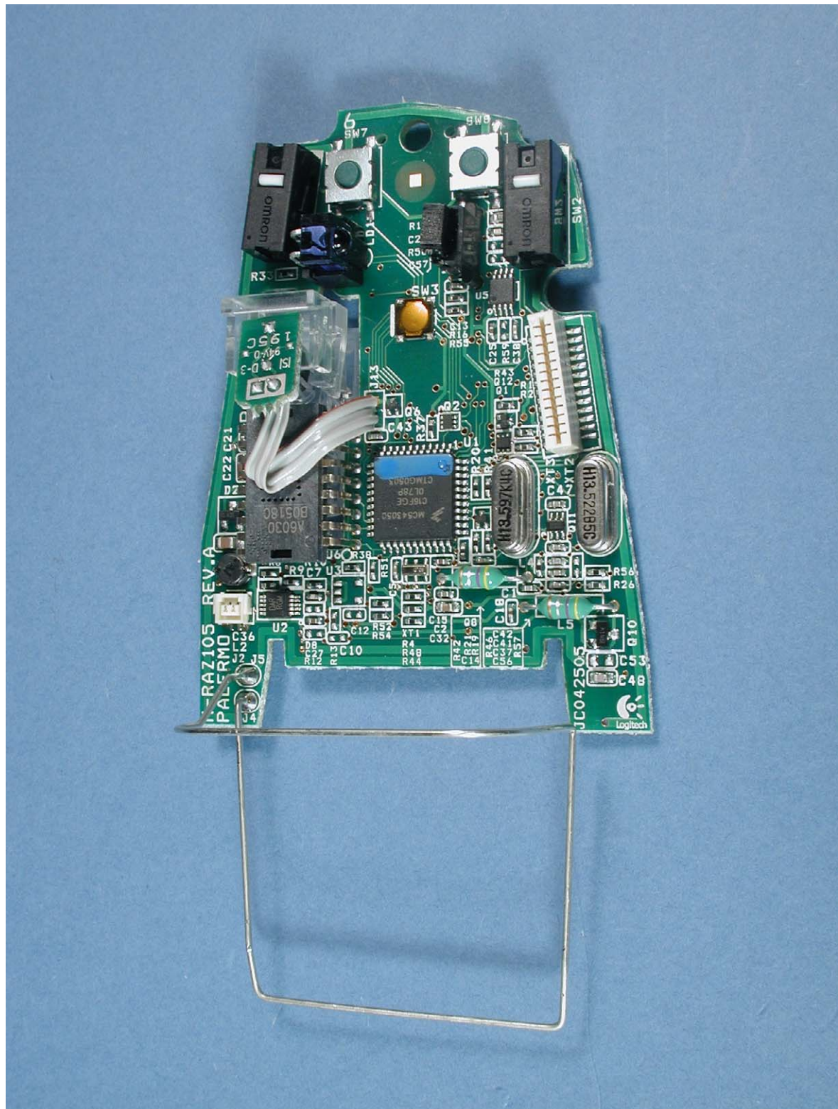
Photograph 7: Top view of M-RAZ105 PCB
