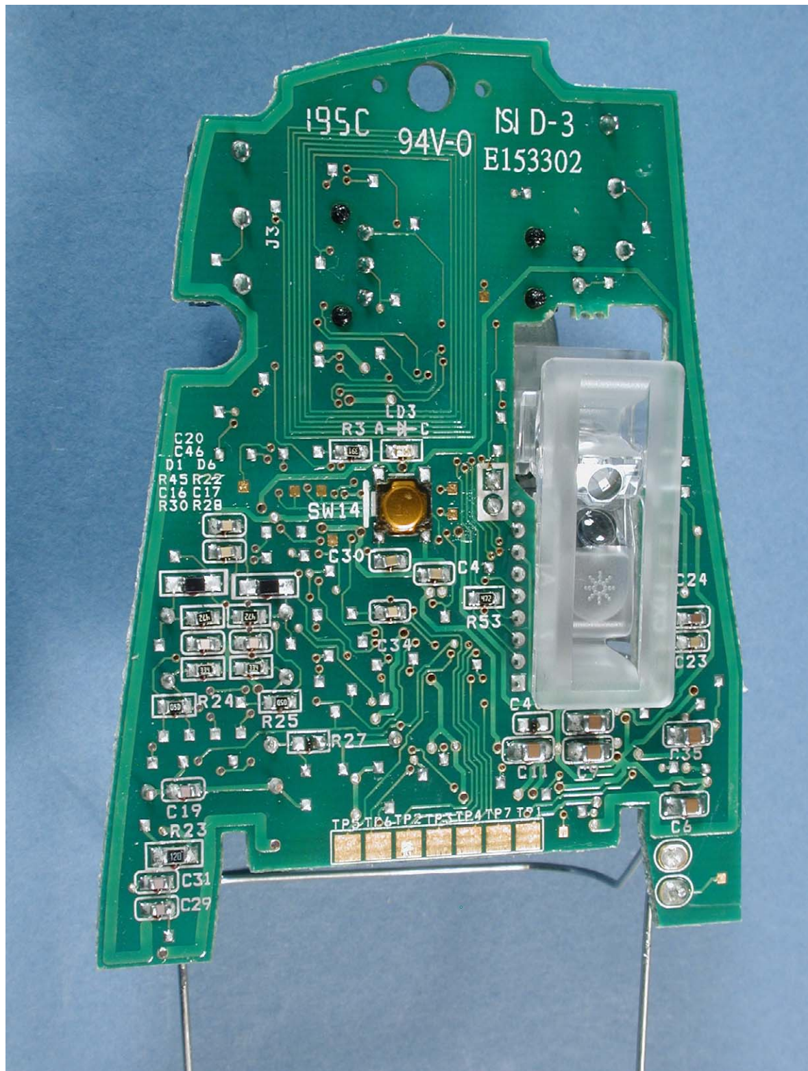
Photograph 8: Bottom view of M-RAZ105 PCB
