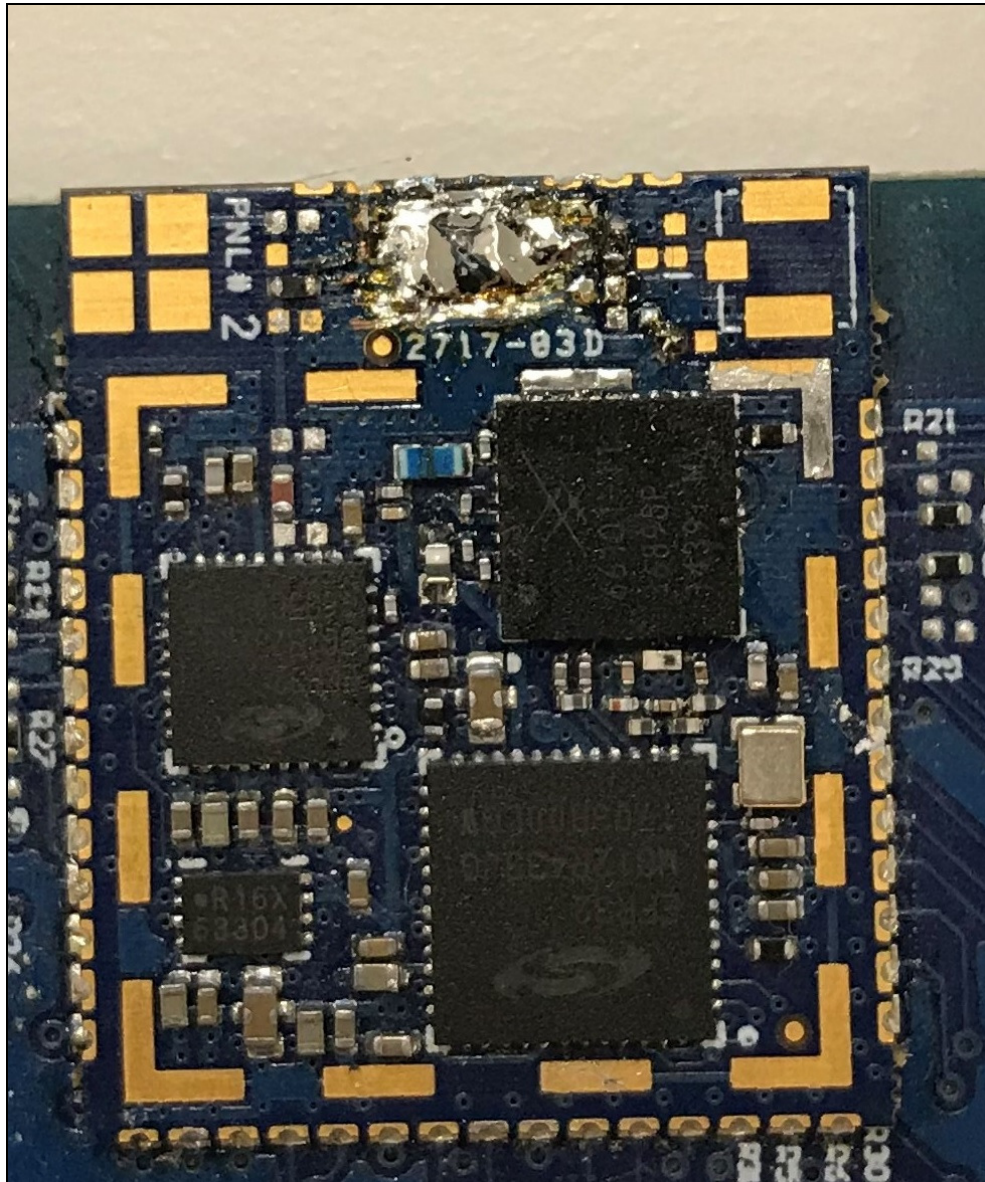
Figure 1: Internal Photo – Shield Removed
