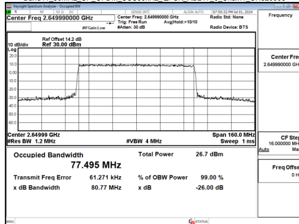
Band41 80MHz CP OFDM SCS30kHz QPSK RB217_0 Chain1 CH529998
