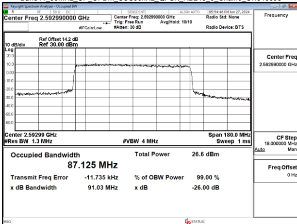
Band41_90MHz_CP_OFDM_SCS30kHz_QPSK_RB245_0_Chain0_CH518598
