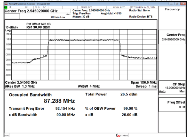
Band41_90MHz_CP_OFDM_SCS30kHz_QPSK_RB245_0_Chain1_CH509004
