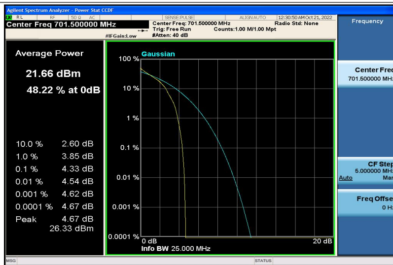
Band12-5MHz-QPSK-23035-1RB#0
