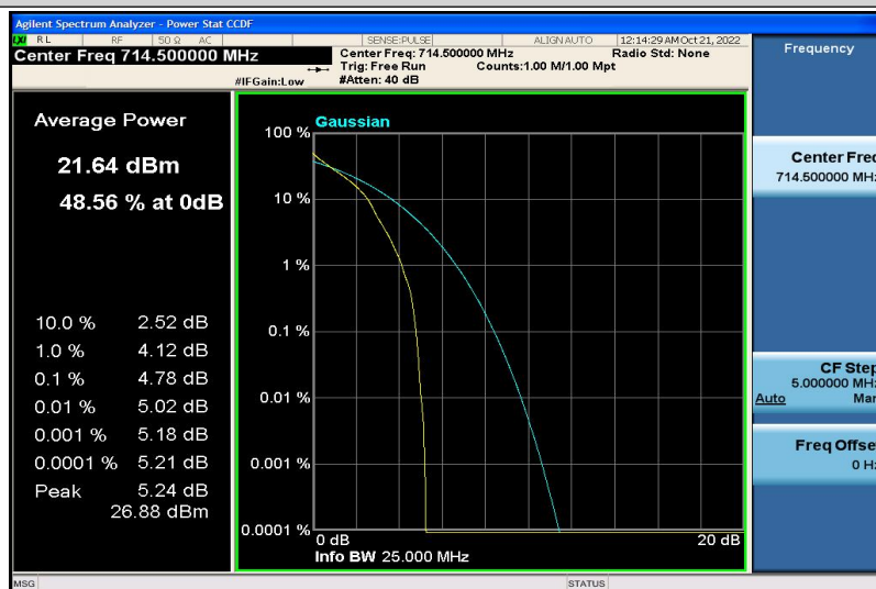
Band12-3MHz-QPSK-23165-1RB#0
