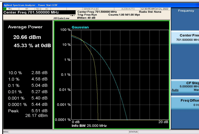
Band12-5MHz-16QAM-23035-1RB#0
