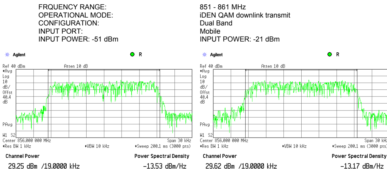
Plot 7.1.20 RF output power measurements at mid frequency carrier, Port 1
