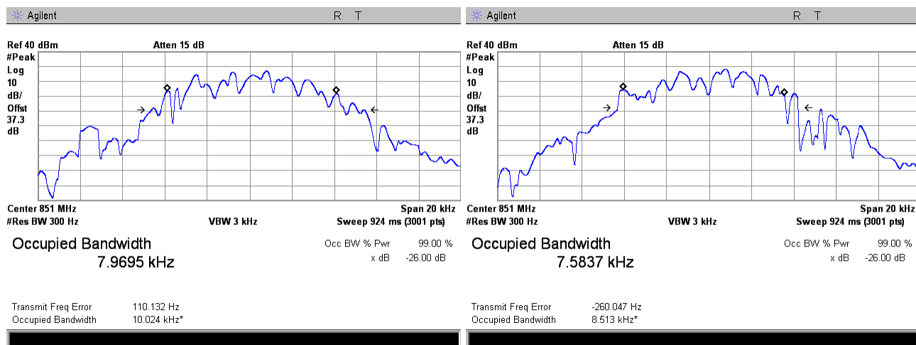
Plot 7.2.8 Occupied bandwidth test result at mid frequency carrier, Port 1
