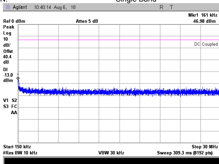
Plot 7.8.54 Spurious emission measurements in 0.15 - 30.0 MHz range at high carrier frequency
