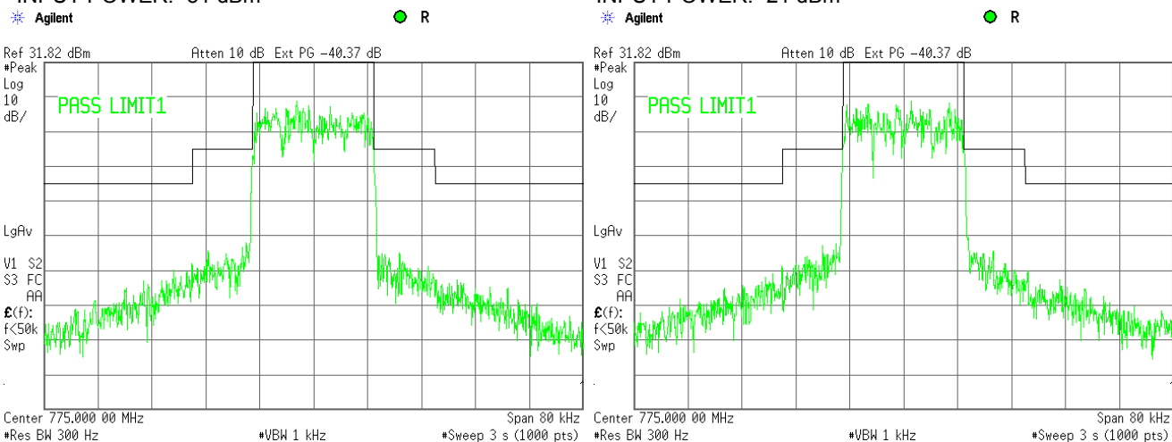
Plot 7.3.28 Emission mask test result at low frequency carrier, Port 2
