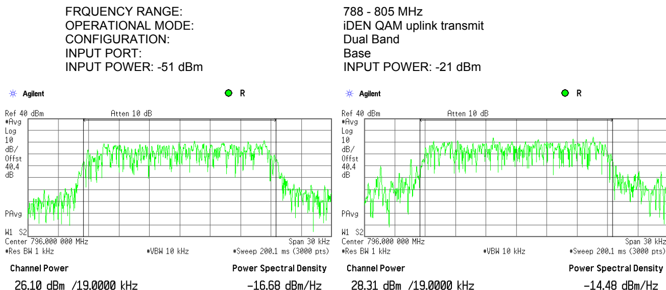
Plot 7.1.17 RF output power measurements at mid frequency carrier, Port 2
