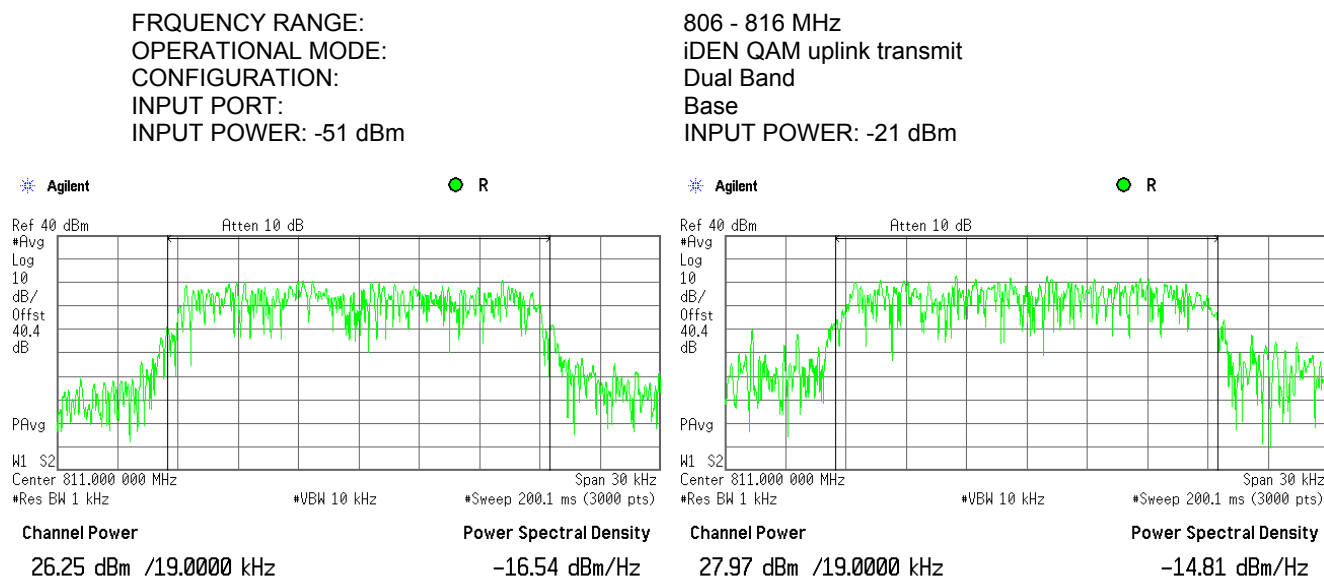
Plot 7.1.23 RF output power measurements at mid frequency carrier, Port 2
