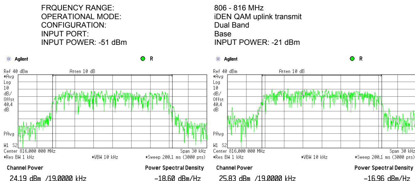
Plot 7.1.24 RF output power measurements at high frequency carrier, Port 2
