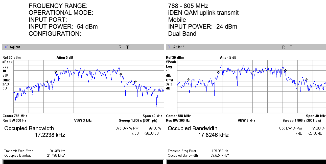
Plot 7.2.16 Occupied bandwidth test result at low frequency carrier, Port 2
