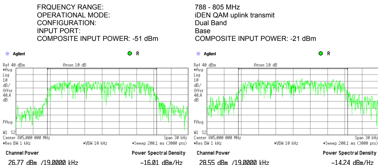
Plot 7.1.18 RF output power measurements at high frequency carrier, Port 2
