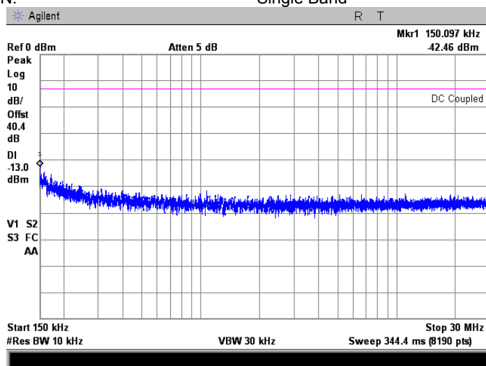
Plot 7.8.102 Spurious emission measurements in 0.15 - 30.0 MHz range at high carrier frequency
