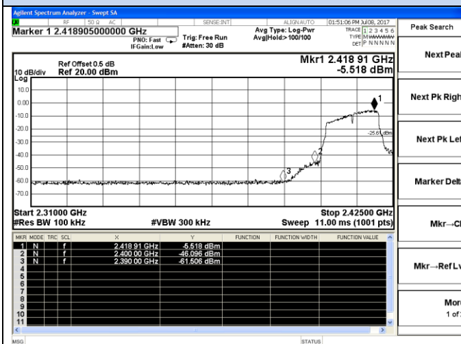
802.11g-Low channel
