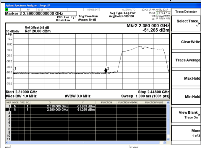
802.11n-HT40-Low channel(Peak)
