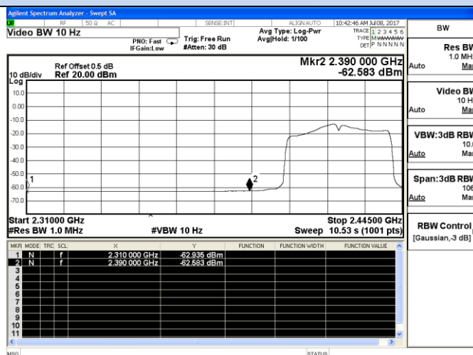
802.11n-HT40-Low channel(Average)
