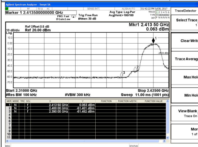
802.11b-Low channel
