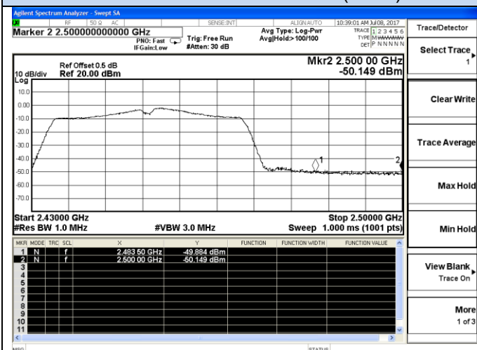
802.11n-HT40-High channel(Peak)
