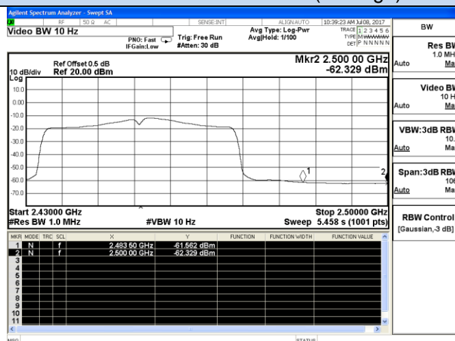
802.11n-HT40-High channel(Average)
