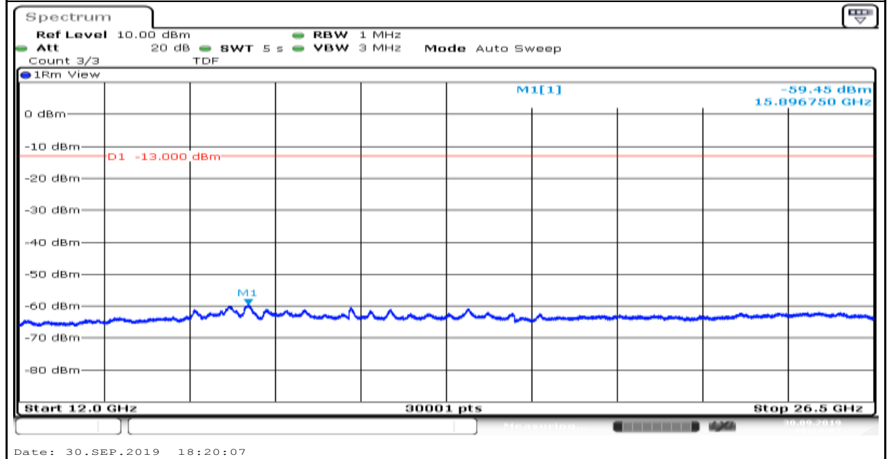
Band85_5MHz_QPSK_134157_3
