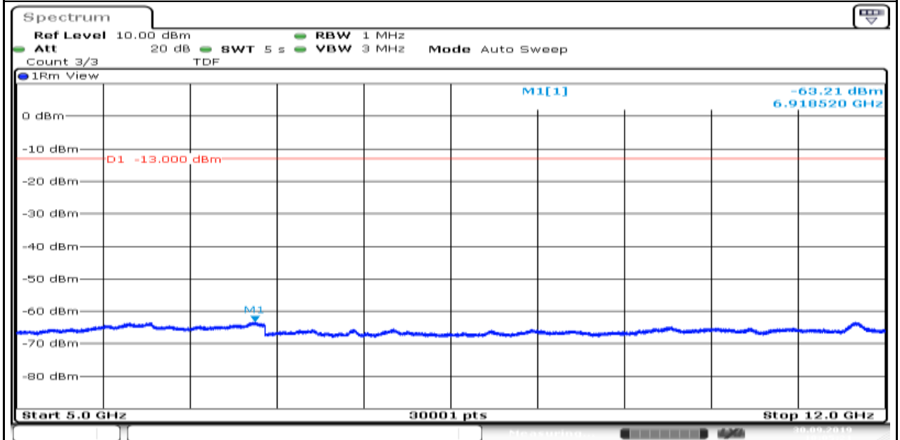
Band85_5MHz_16QAM_134092_1
