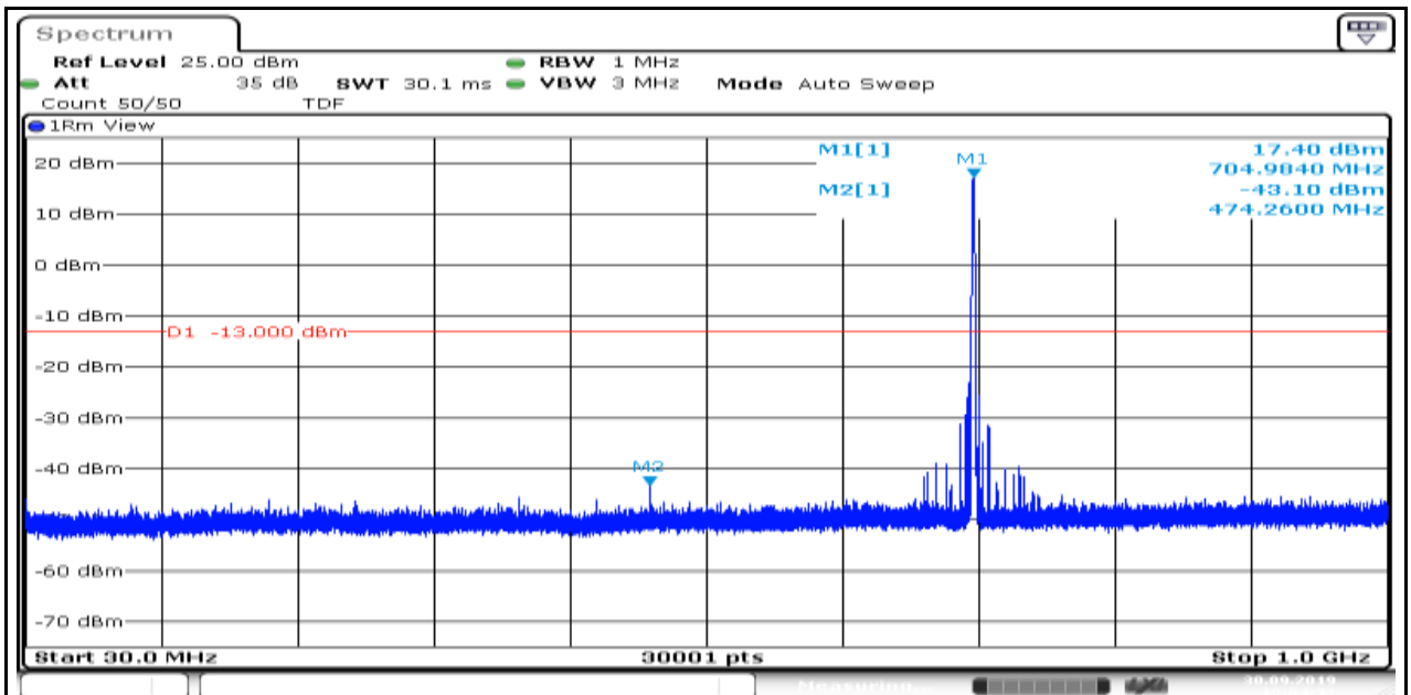
Band85_5MHz_16QAM_134092_1
