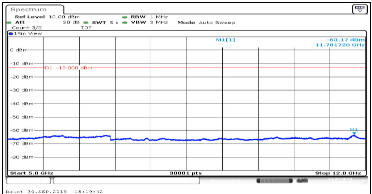
Band85_5MHz_QPSK_134157_3
