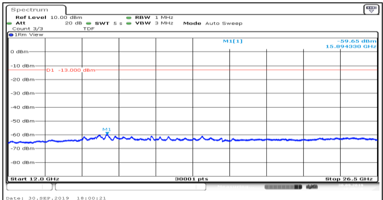
Band85_5MHz_QPSK_134027_6
