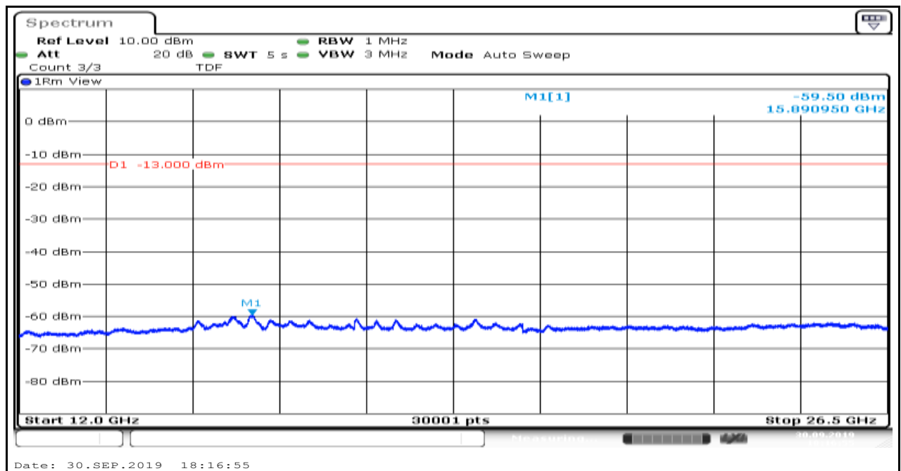
Band85_5MHz_QPSK_134157_3
