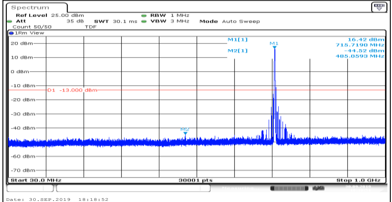
Band85_5MHz_QPSK_134157_1
