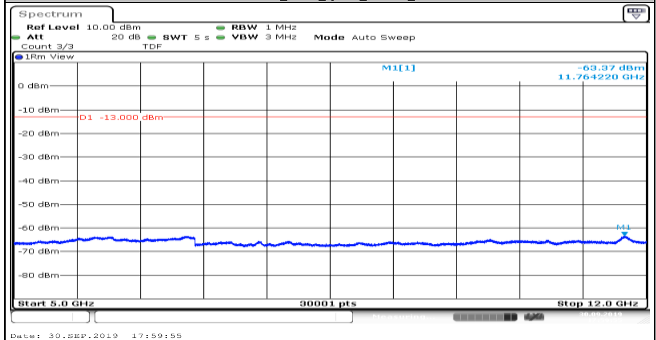
Band85_5MHz_QPSK_134027_6
