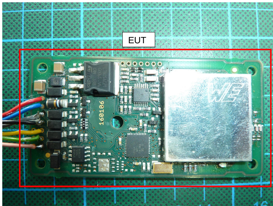
170664eut3: EUT bottom view with shielding
