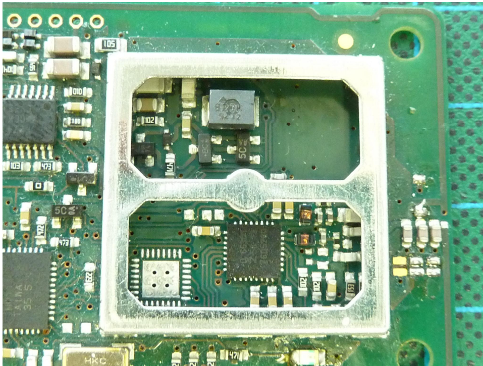
170664eut5: EUT detail view 1
