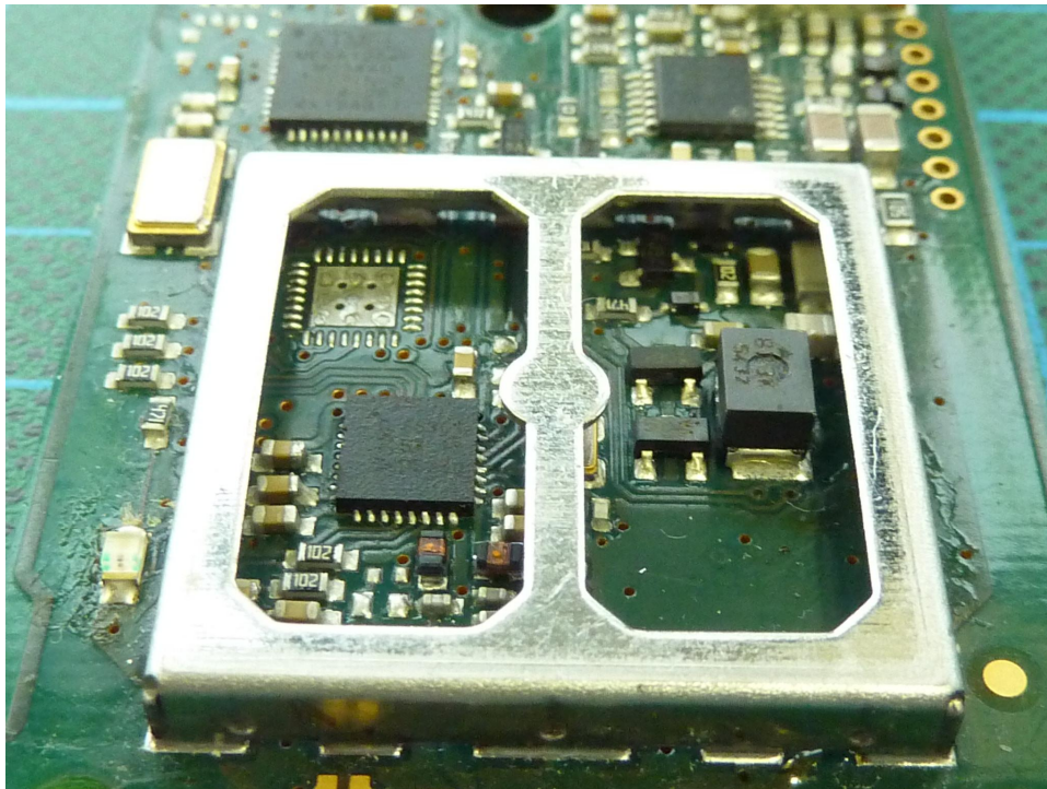
170664eut8: EUT detail view 3
