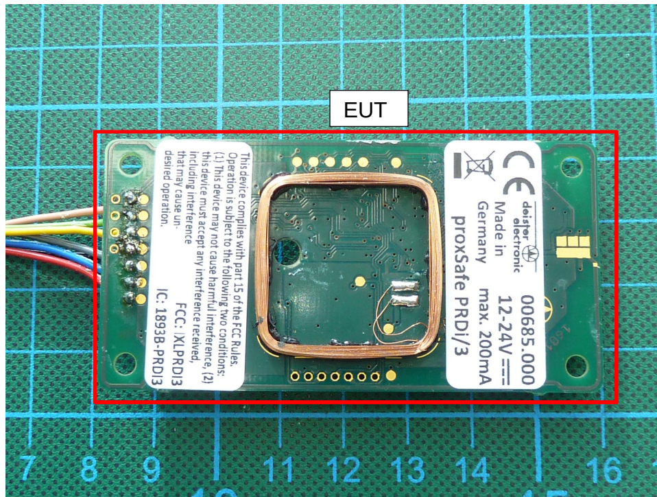
170664eut1: EUT top view with label
