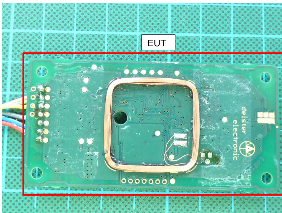
170664eut2: EUT top view without label
