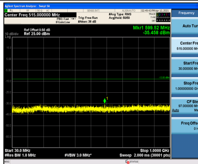
Band4-10MHz-QPSK-20350-1-0-High-30-1000
