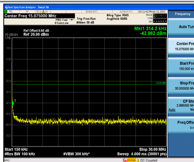
Band4-5MHz-16QAM-19975-1-0-Low-0.15-30
