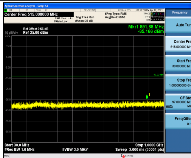
Band4-10MHz-16QAM-20000-1-0-Low-30-1000
