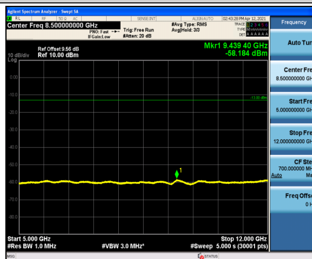
Band4-10MHz-16QAM-20000-1-0-Low-5000-12000
