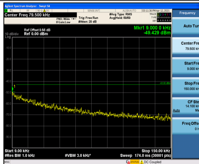
Band4-5MHz-16QAM-19975-1-0-Low-0.009-0.15
