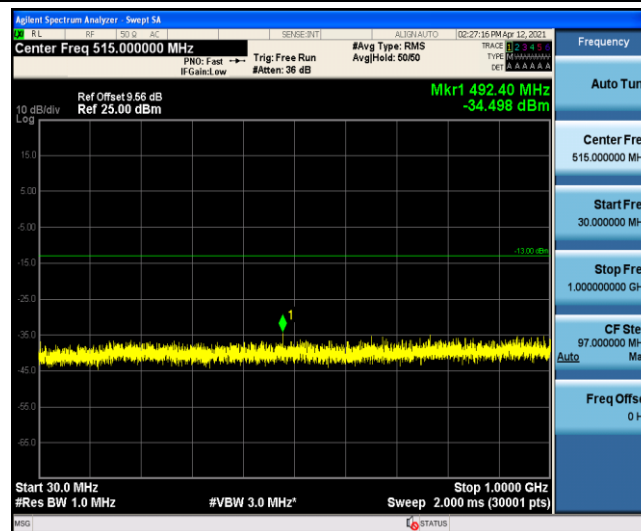
Band4-10MHz-QPSK-20175-1-0-Low-30-1000
