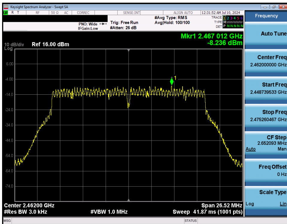
Plot 7-117. Power Spectral Density Plot Antenna WF7 (802.11n (2.4GHz) – Ch. 11) – MCS7
