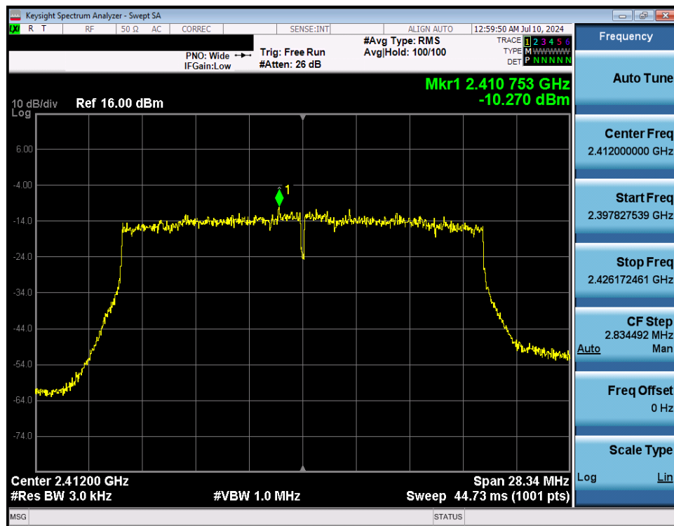
Plot 7-152. Power Spectral Density Plot CDD Antenna WF7 (802.11ax (SU - 2.4GHz) – Ch. 1) – MCS4
