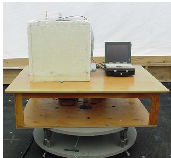
Photograph E.7-4 - Front of Radiated Emission Setup with vehicle-mount antenna and cradle
