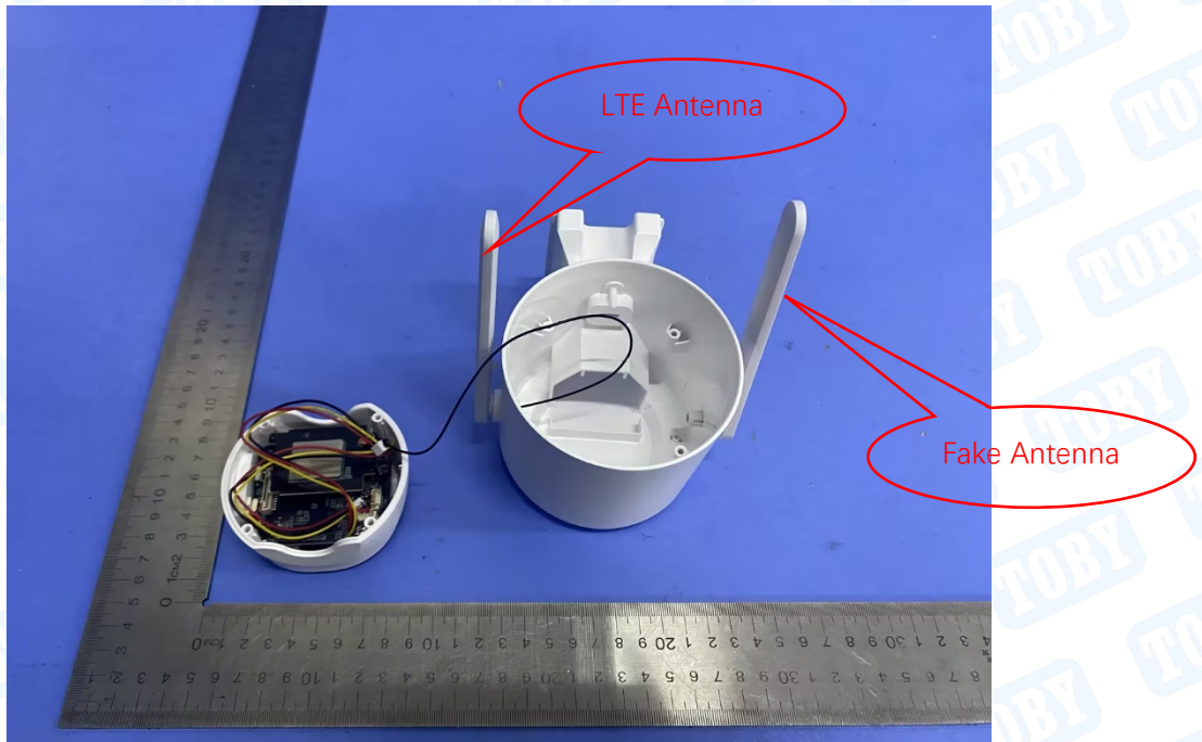
Photo 13 Internal of EUT
