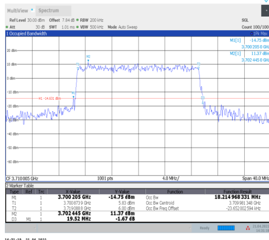
1-N77-3700-3980--30-20-L-8-CP-64QAM-Outer_Full- 51@0-Ant0-18.215-19.520-≤20-PASS
