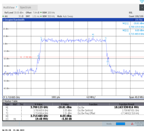
1-N77-3700-3980--30-20-L-9-CP-256QAM-Outer_Fu ll-51@0-Ant0-18.164-19.480-≤20-PASS
