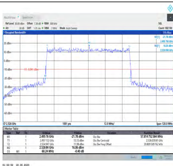
1-N41-PC1-30-60-L-1-DFT-QPSK-Outer_Full-162@0 -Ant1-57.815-60.240-≤60-PASS
