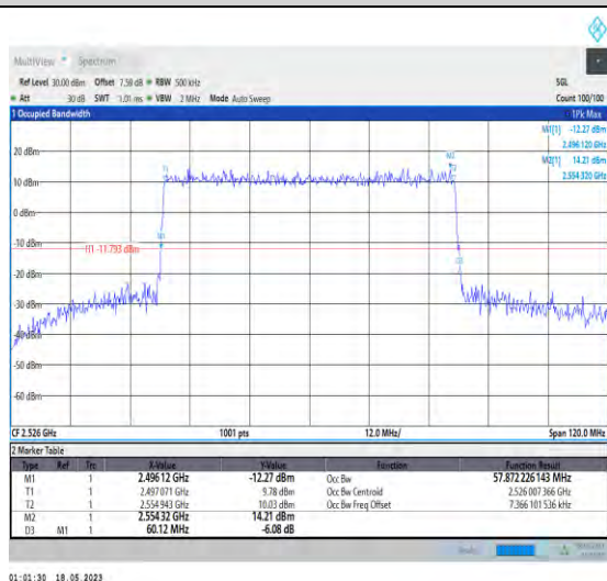
1-N41-PC1-30-60-L-3-DFT-16QAM-Outer_Full-162@0-Ant1-57.872-60.120-≤60-PASS
