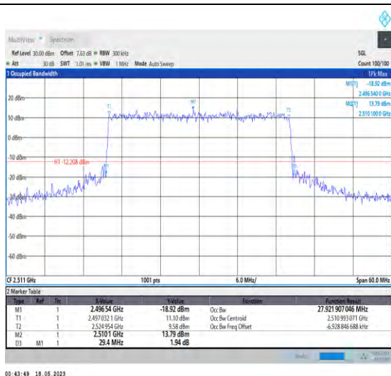
1-N41-PC1-30-30-L-6-CP-QPSK-Outer_Full-78@0-Ant1-27.922-29.400-≤30-PASS
