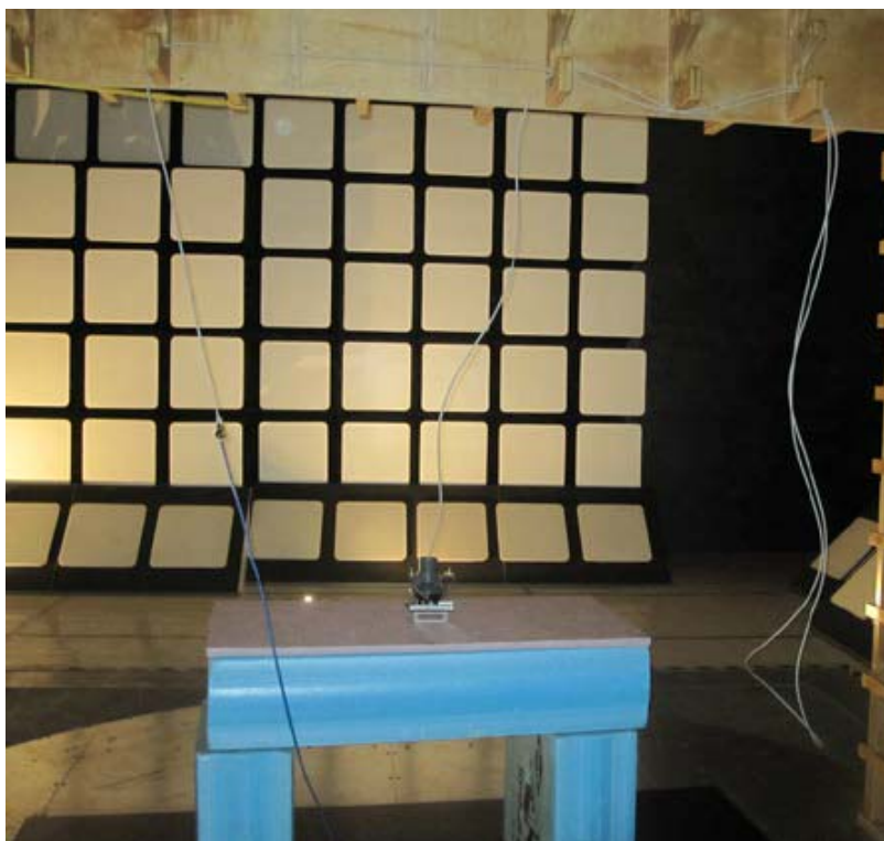
EUT Set Up
