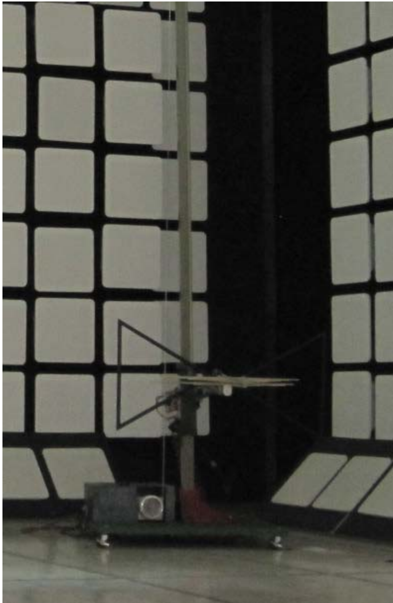
Receive Antenna
