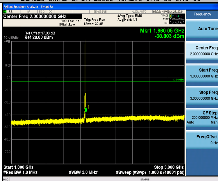
Band25_3MHz_QPSK_26055_15RB#0_1000~3000_1000~3000
