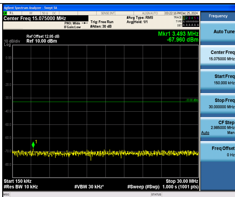
Band25_3MHz_QPSK_26055_15RB#0_0.15~30_0.15~30
