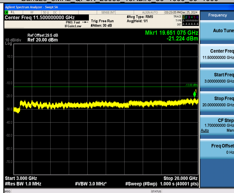
Band25_3MHz_QPSK_26055_15RB#0_3000~20000_3000~20000
