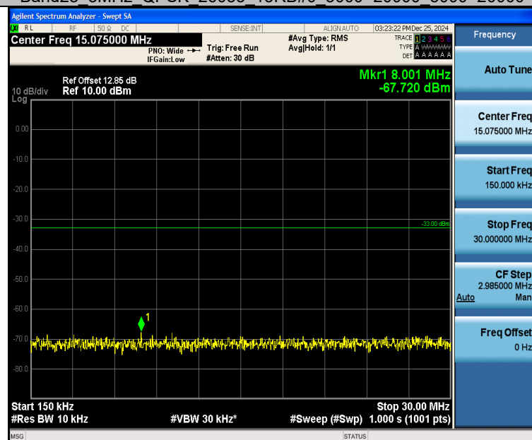
Band25_3MHz_16QAM_26055_15RB#0_0.15~30_0.15~30
