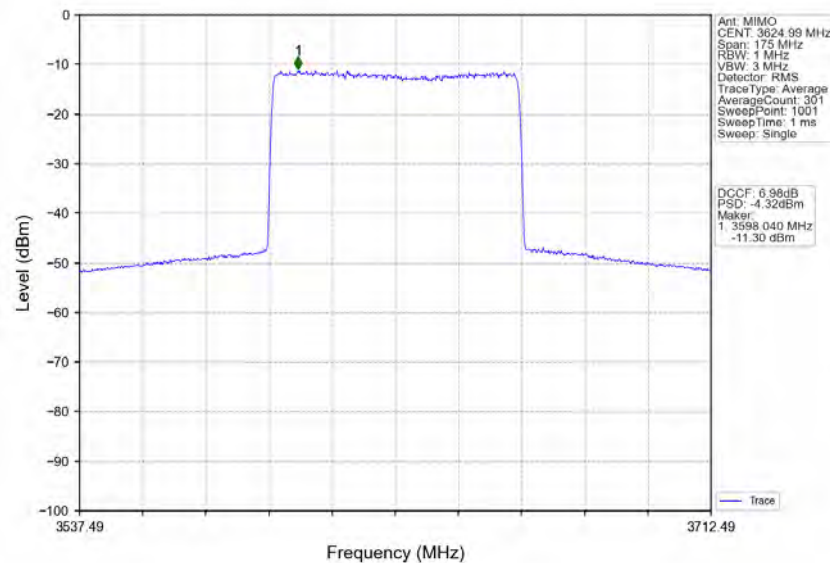
n78d_30kHz_MIMO_NTNV_70MHz_CP-OFDM_256_QAM_3624.99MHz_Inner_Full
