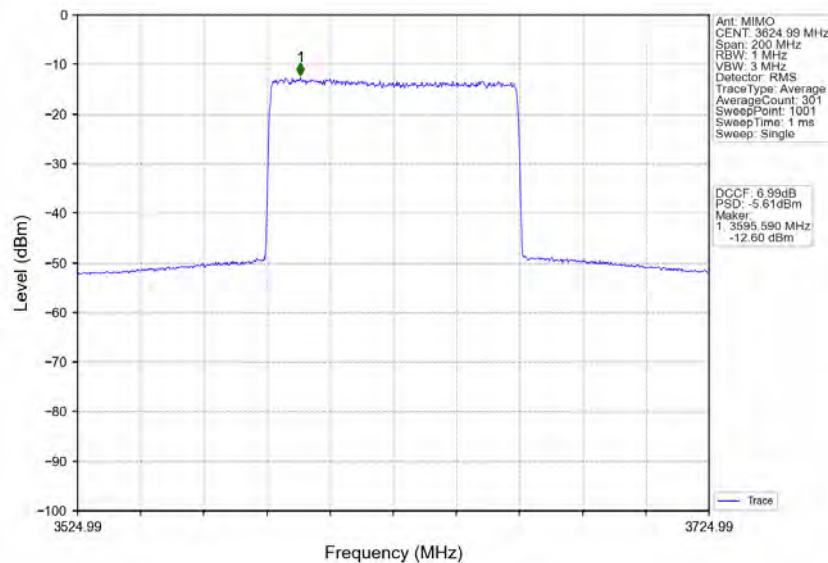
n78d_30kHz_MIMO_NTNV_80MHz_CP-OFDM_QPSK_3624.99MHz_Inner_Full
