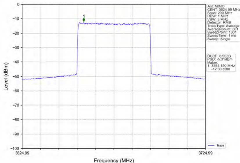
n78d_30kHz_MIMO_NTNV_80MHz_CP-OFDM_16_QAM_3624.99MHz_Inner_Full
