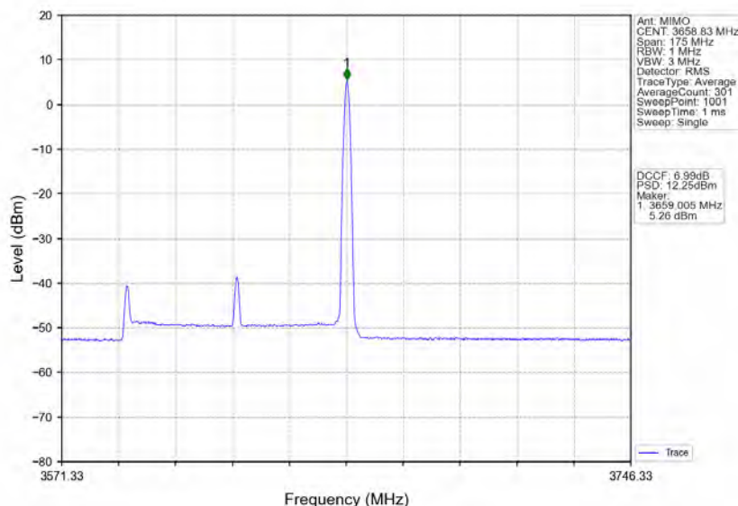
n78d_30kHz_MIMO_NTNV_70MHz_CP-OFDM 16 QAM_3624.99MHz_Edge_1RB_Right
