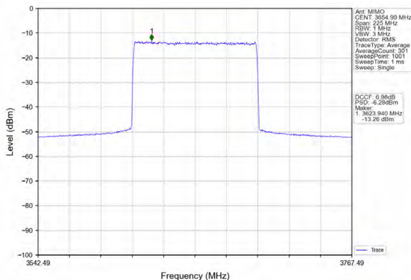
n78d_30kHz_MIMO_NTNV_90MHz_CP-OFDM 64 QAM_3654.99MHz_Inner_Full
