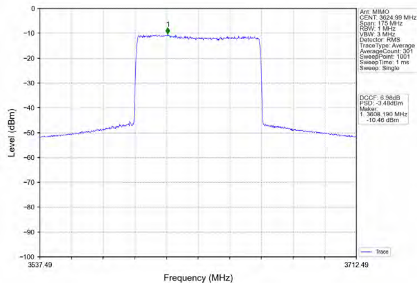
n78d_30kHz_MIMO_NTNV_70MHz_CP-OFDM 64 QAM_3624.99MHz_Inner_Full
