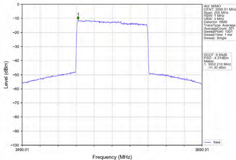
n78d_30kHz_MIMO_NTNV_80MHz_CP-OFDM_256_QAM_3590.01MHz_Inner_Full
