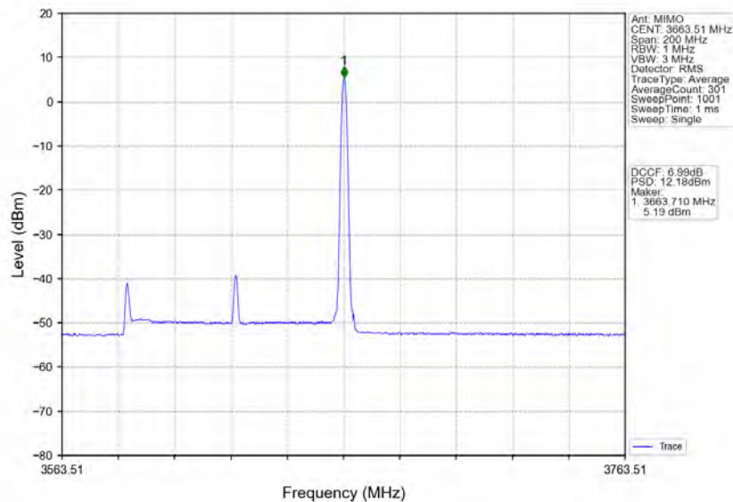
n78d_30kHz_MIMO_NTNV_80MHz_CP-OFDM 16 QAM_3624.99MHz_Inner_1RB_Right
