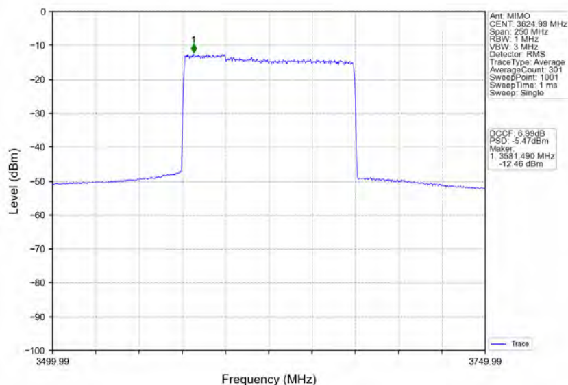
n78d_30kHz_MIMO_NTNV_100MHz_CP-OFDM QPSK_3624.99MHz_Inner_Full
