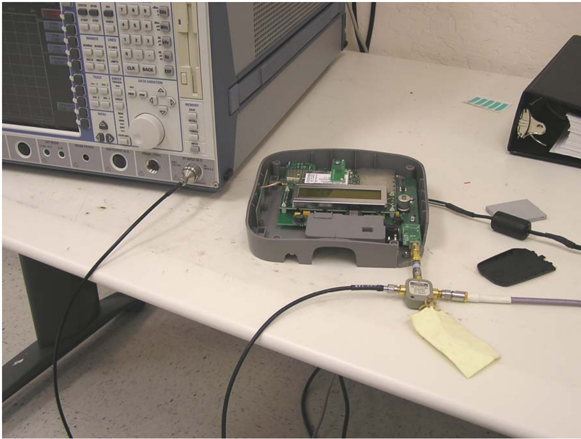
Test setup – Conducted measurements for BT
