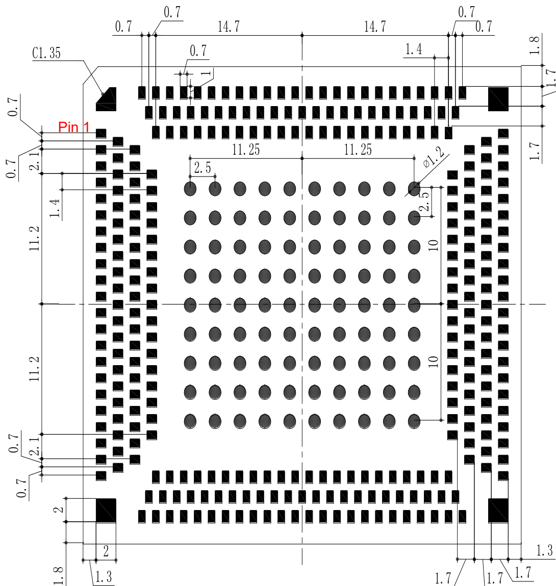
Figure 50: Recommended Footprint
