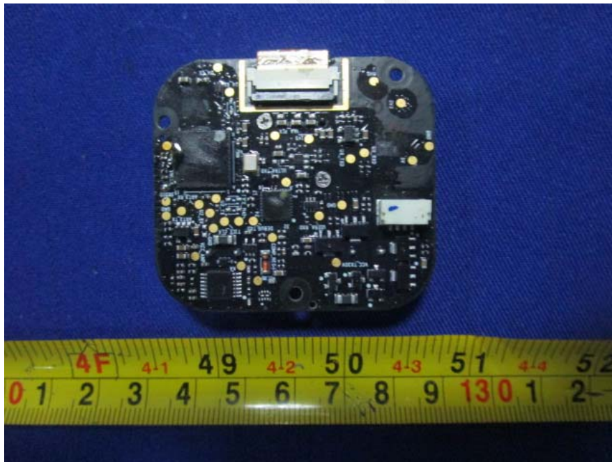
EUT –RF Module Sub board Bottom View
