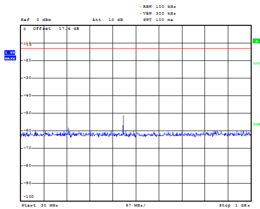
GSM 1900 CH-Low 30MHz~1GHz
