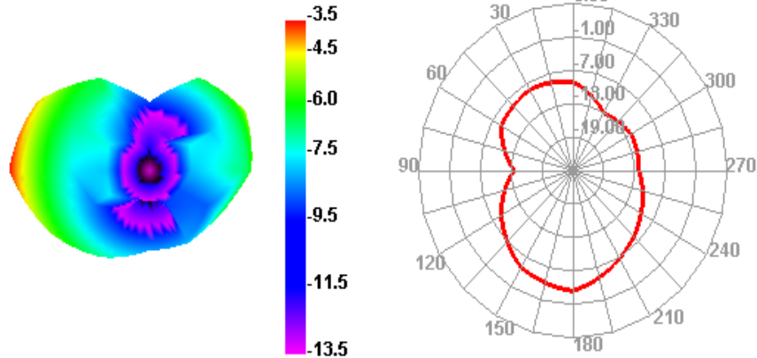
Bluetooth 0 TRP H
