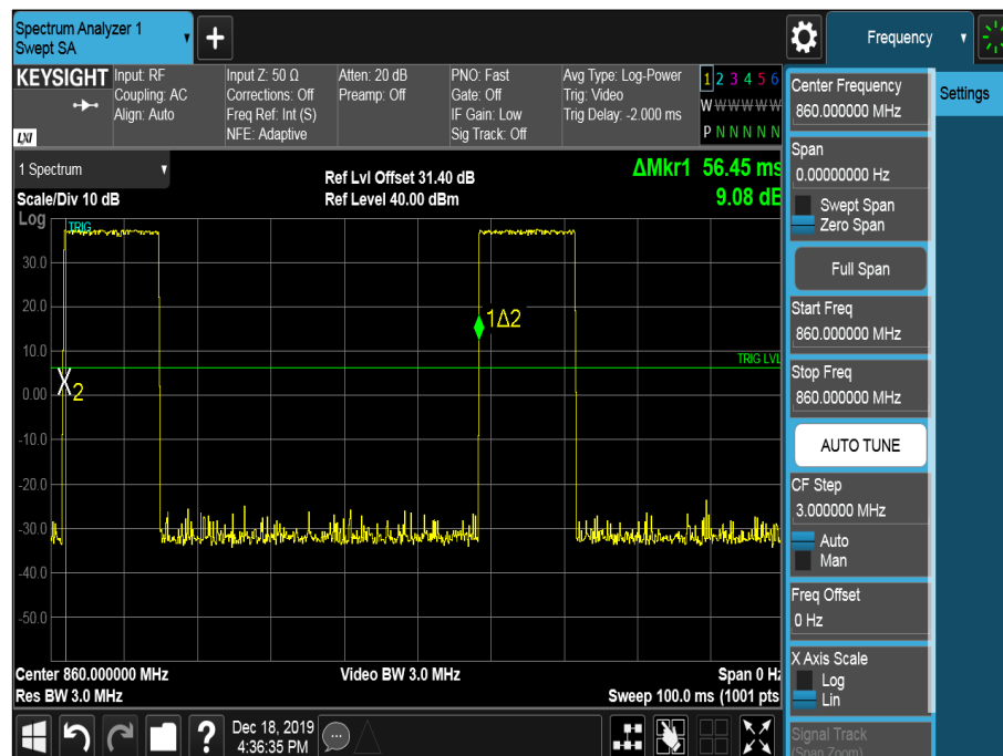
Figure 59 - Burst Period
