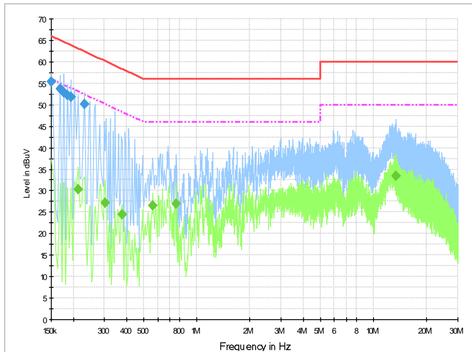
Fig.B.8.1 AC Powerline Conducted Emission- bluetooth
