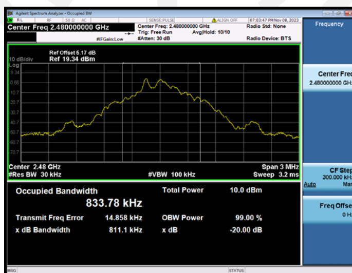
GFSK(1-DH1) 2480MHz
