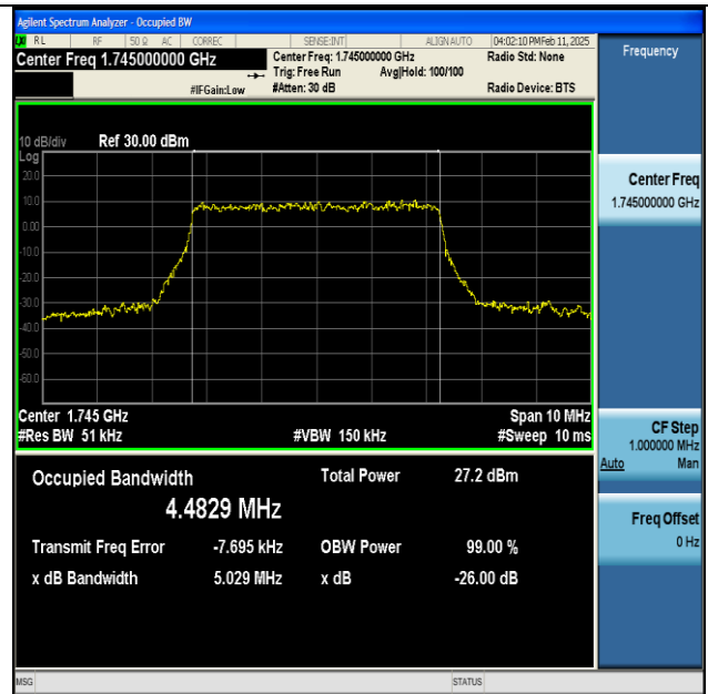
NTNV-n66-PC3-15-5-M-DFT-256QAM-Outer_Full-Ant1- PASS
