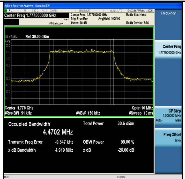
NTNV-n66-PC3-15-5-H-DFT-QPSK-Outer_Full-Ant1-PASS
