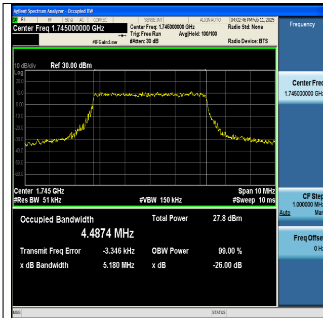
NTNV-n66-PC3-15-5-M-CP-64QAM-Outer_Full-Ant1- PASS
