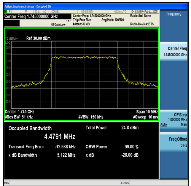
NTNV-n66-PC3-15-5-M-CP-256QAM-Outer_Full-Ant1- PASS
