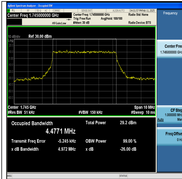
NTNV-n66-PC3-15-5-M-DFT-64QAM-Outer_Full-Ant1- PASS
