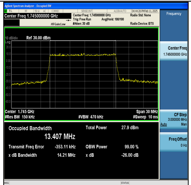
NTNV-n66-PC3-15-15-M-DFT-256QAM-Outer_Full-Ant1- PASS
