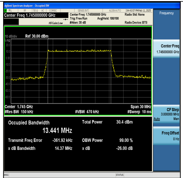
NTNV-n66-PC3-15-15-M-DFT-16QAM-Outer_Full-Ant1- PASS
