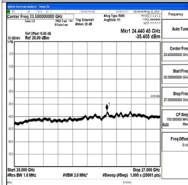
Band41_20MHz_QPSK_41490_1RB#0_20000~27000_20000~27000
