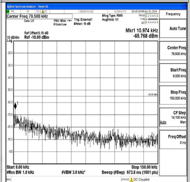
Band41_20MHz_16QAM_41490_1RB#0_0.009~0.15_0.009~0.15
