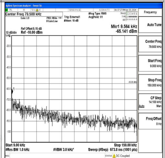
Band41_20MHz_16QAM_39750_1RB#0_0.009~0.15_0.009~0.15
