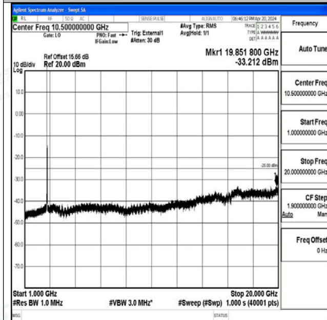
Band41_20MHz_16QAM_41490_1RB#0_1000~20000_1000~20000
